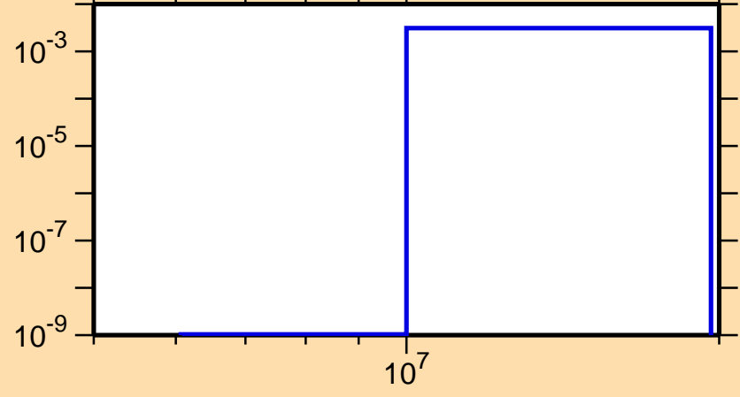
\sigma vs. E for ^{85}\text{Y}(n,n\alpha)
