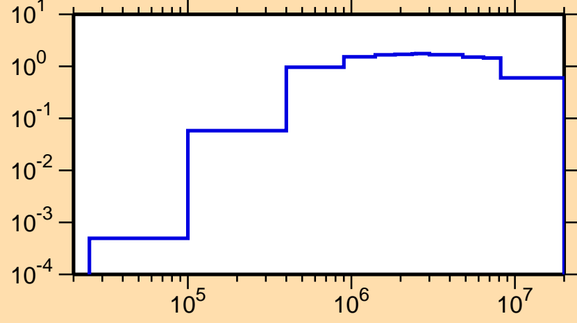
\sigma vs. E for ^{85}\text{Y}(n,\text{inel.})
