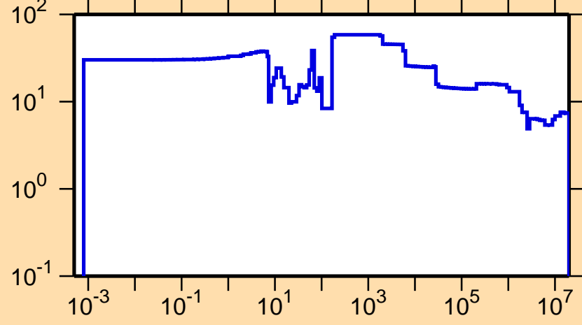
\Delta\sigma/\sigma vs. E for ^{85}\text{Y}(n,\text{tot.})
