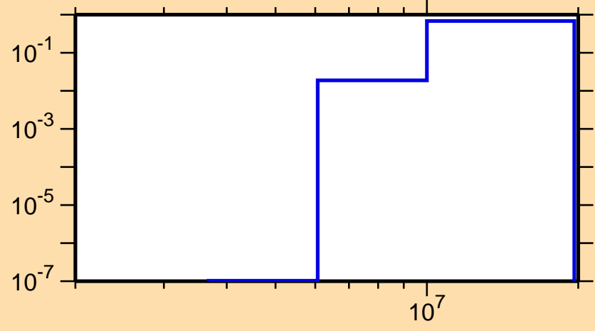
\sigma vs. E for ^{85}\text{Y}(n,np)
