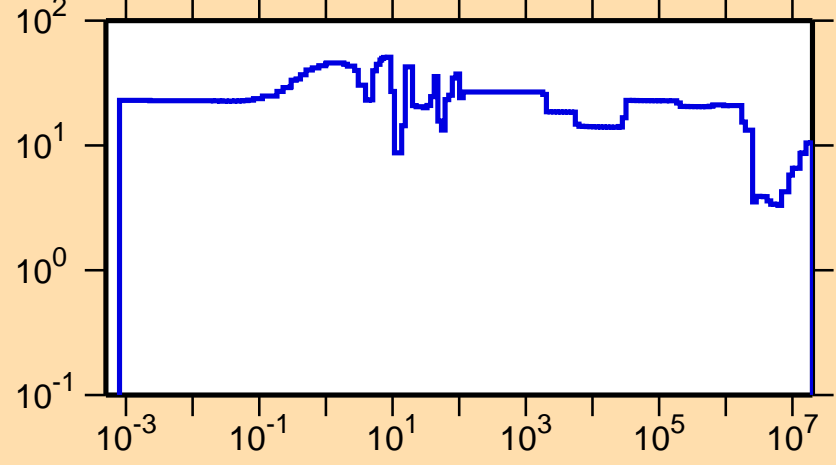
\Delta\sigma/\sigma vs. E for ^{86}\text{Y}(n,\text{tot.})
