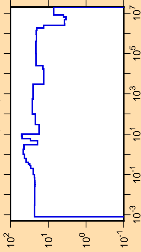
\Delta\sigma/\sigma vs. E for ^{86}\text{Y}(n,\text{tot.})
