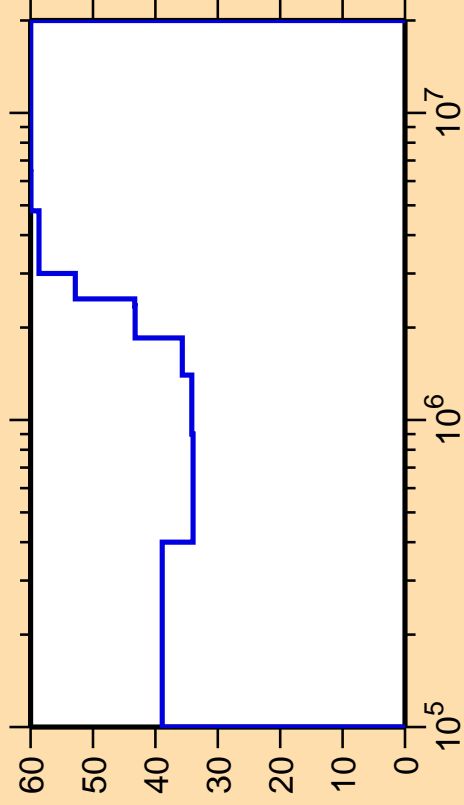
\Delta\sigma/\sigma vs. E for ^{86}\text{Y}(n,n_4)
