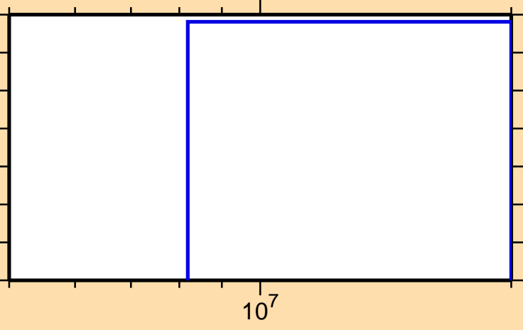
\sigma vs. E for ^{86}\text{Y}(n,\text{He}3)
