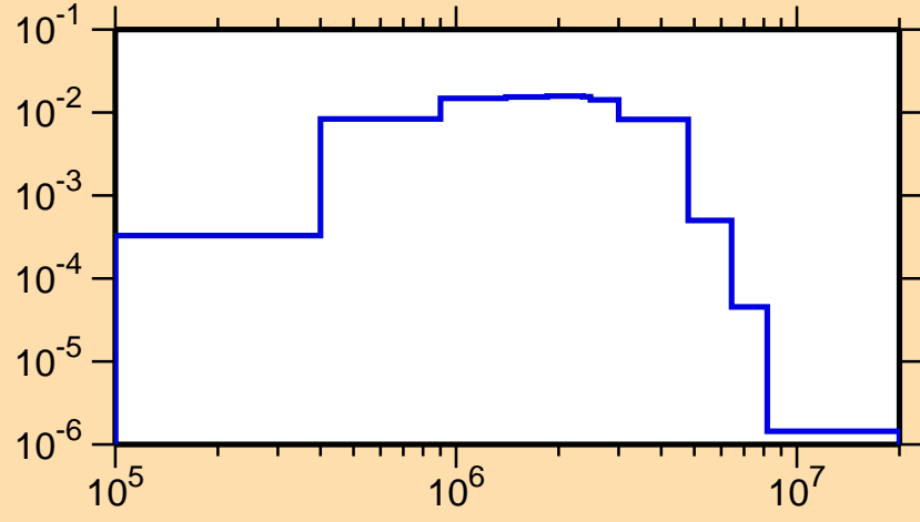
\sigma vs. E for ^{86}\text{Y}(n,n_4)
