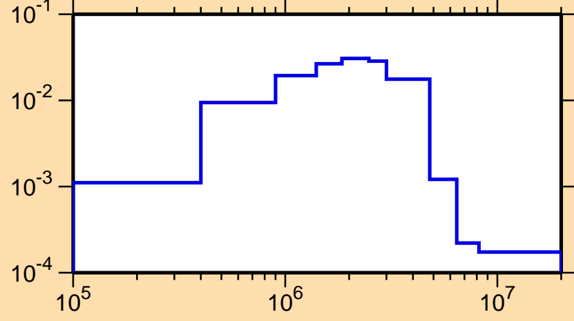
\sigma vs. E for ^{86}\text{Y}(n,n_2)
