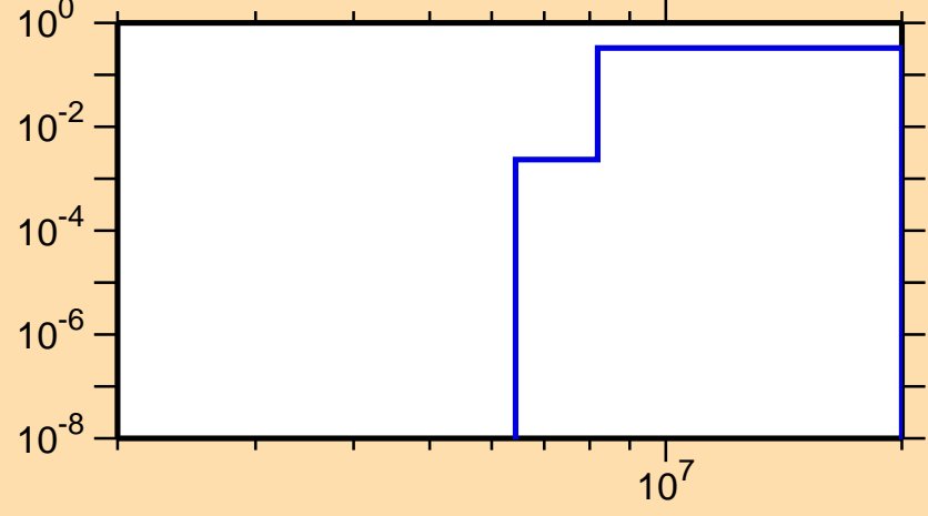
\sigma vs. E for ^{86}\text{Y}(n,np)
