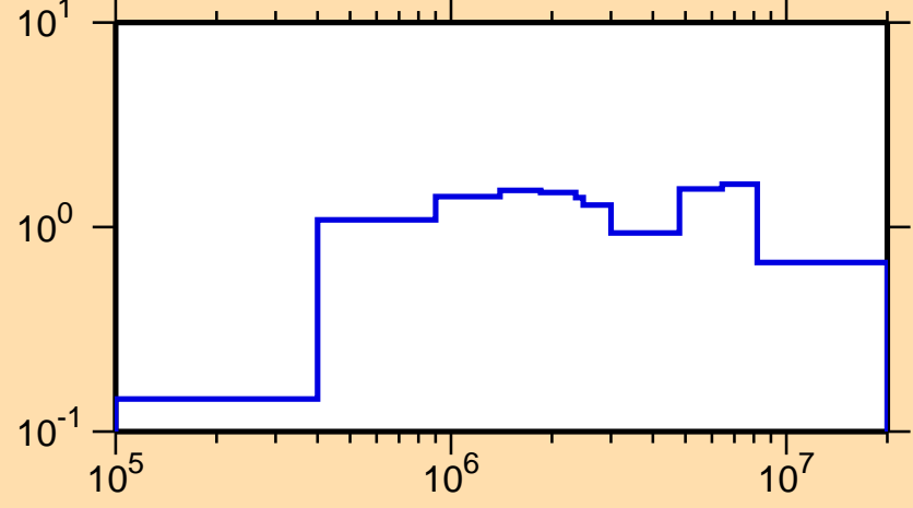
\sigma vs. E for ^{86}\text{Y}(n,\text{inel.})
