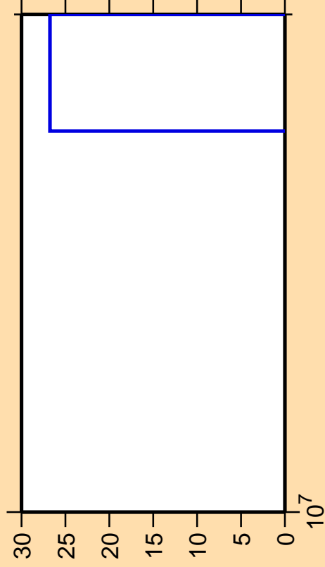
\Delta\sigma/\sigma vs. E for ^{86}\text{Y}(n,nt)
