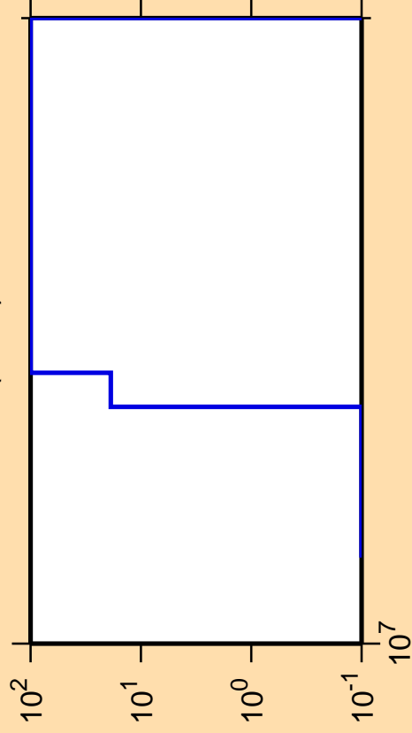
\Delta\sigma/\sigma vs. E for ^{86}\text{Y}(n,nd)
