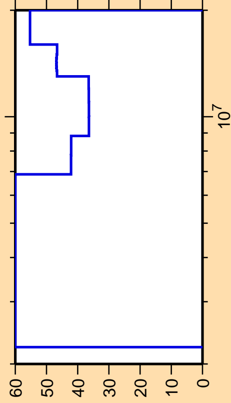
\Delta\sigma/\sigma vs. E for ^{86}\text{Y}(n,p)
