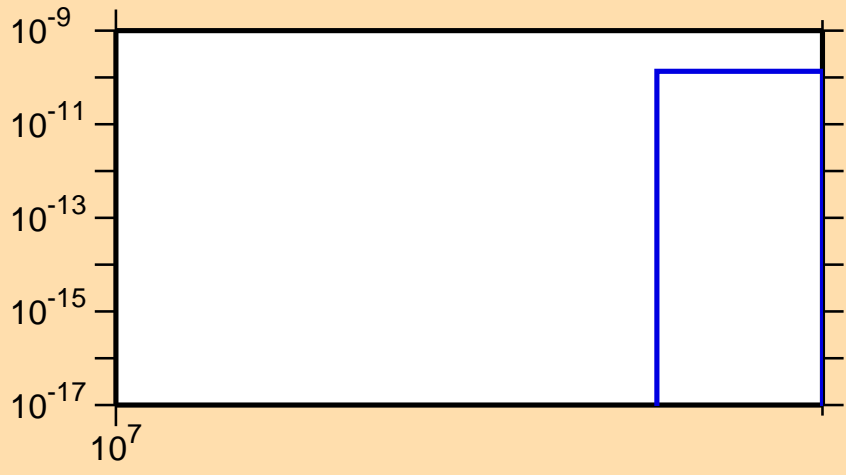
\sigma vs. E for ^{86}\text{Y}(n,\text{pt})
