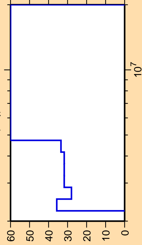
\Delta\sigma/\sigma vs. E for ^{86}\text{Y}(n,\gamma)
