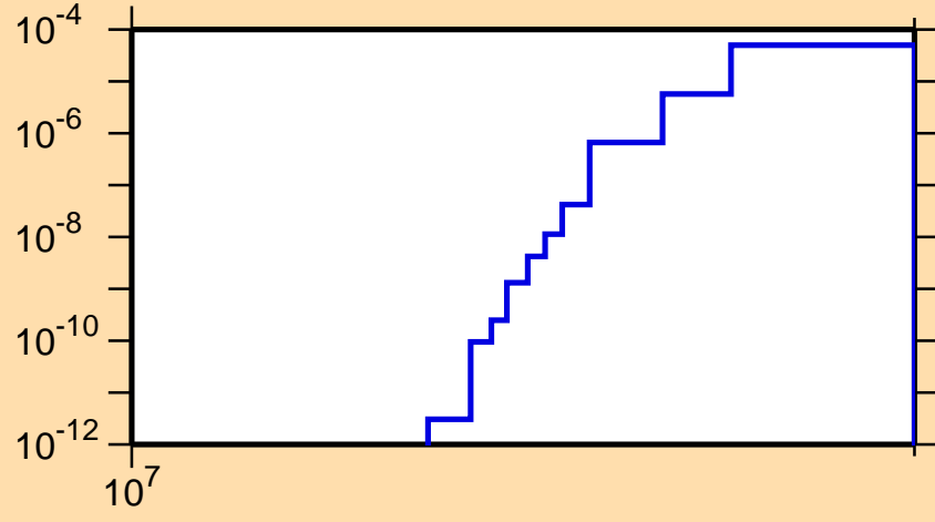
\sigma vs. E for ^{86}\text{Y}(n,nd)
