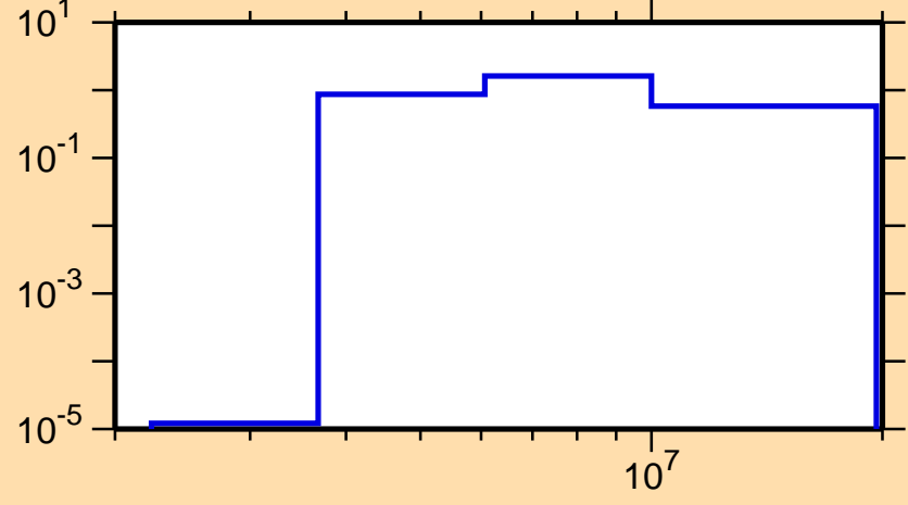
\sigma vs. E for ^{86}\text{Y}(n,n\text{cont.})
