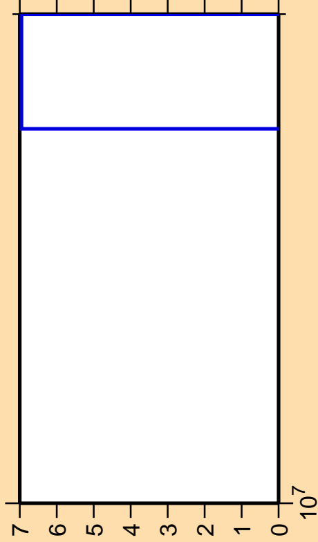
\Delta\sigma/\sigma vs. E for ^{87}\text{Y}(n,nt)
