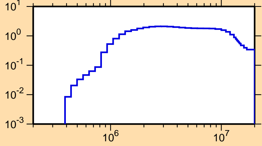
\sigma vs. E for ^{87}\text{Y}(n,\text{inel.})
