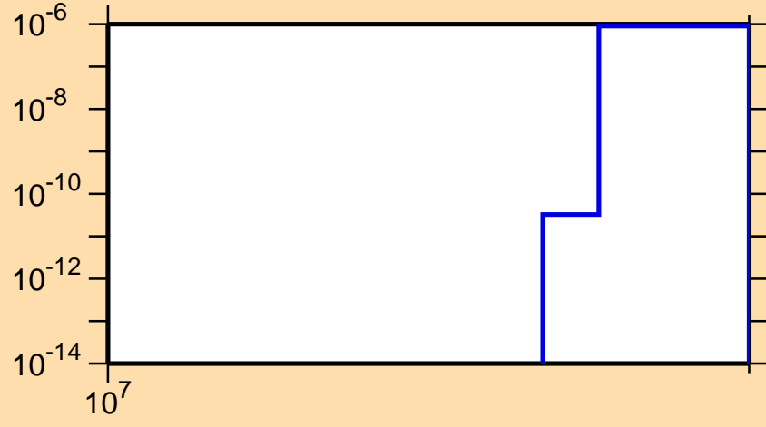
\sigma vs. E for ^{87}\text{Y}(n,nd)
