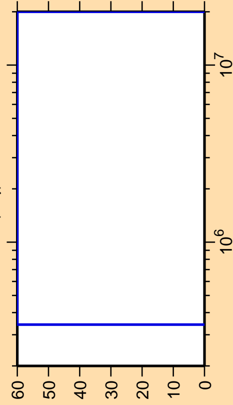
\Delta\sigma/\sigma vs. E for ^{87}\text{Y}(n,\gamma)
