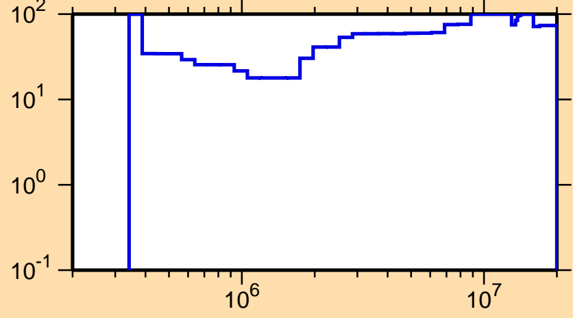
\Delta\sigma/\sigma vs. E for ^{87}\text{Y}(n,n_1)
