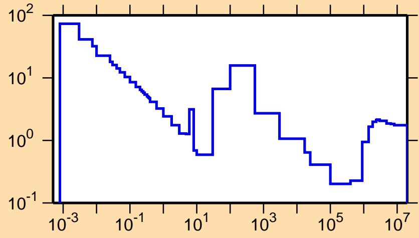
\sigma vs. E for ^{87}\text{Y}(n,\text{nonel.})
