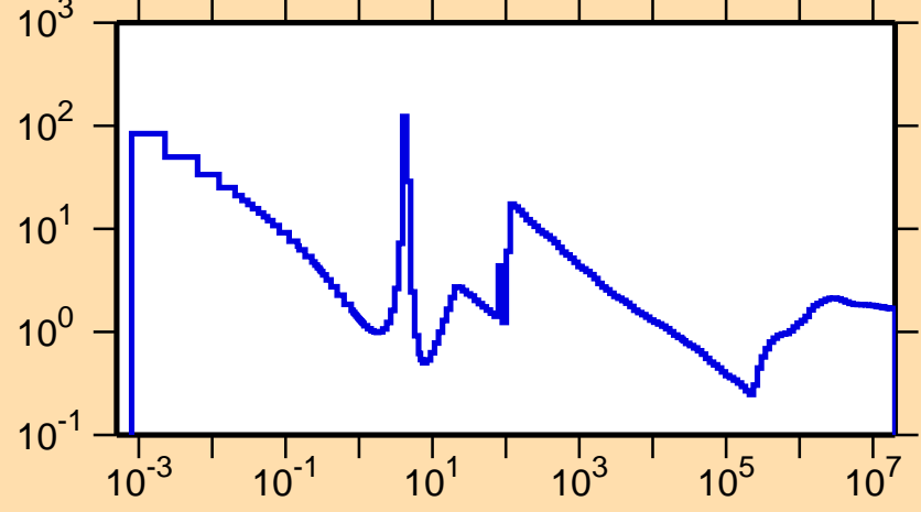
\sigma vs. E for ^{88}\text{Y}(n,\text{nonel.})
