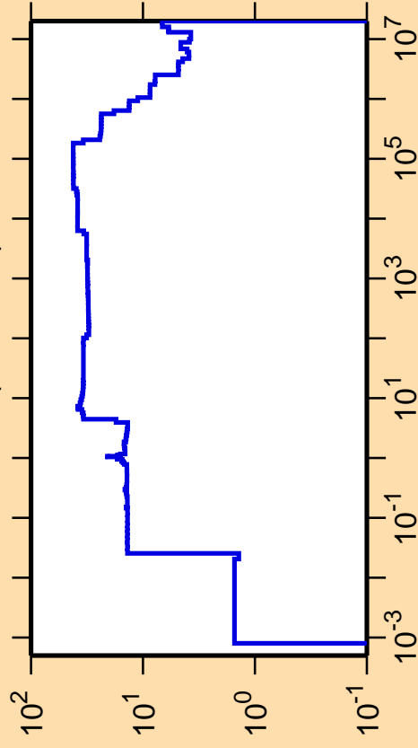
\Delta\sigma/\sigma vs. E for ^{88}\text{Y}(n,\text{nonel.})
