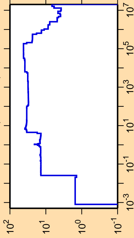
\Delta\sigma/\sigma vs. E for ^{88}\text{Y}(n,\text{nonel.})
