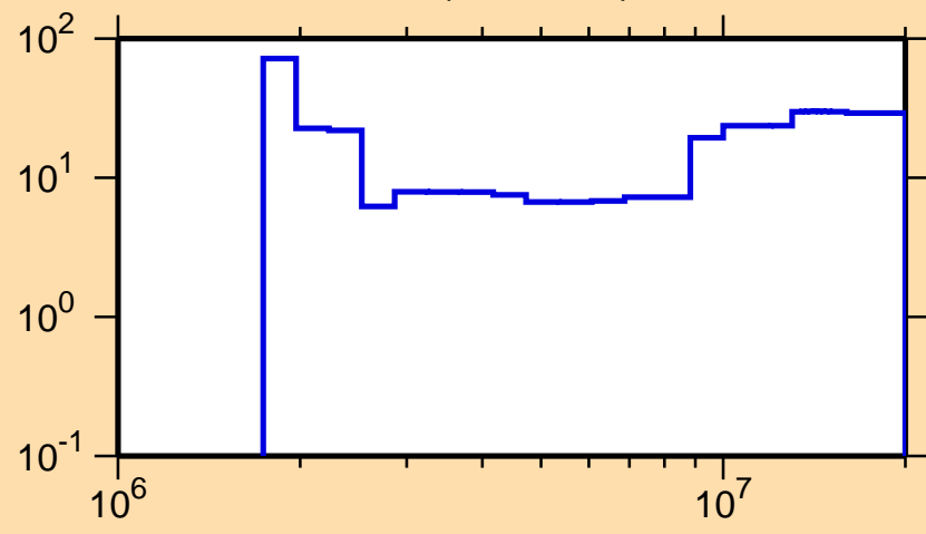
\Delta\sigma/\sigma vs. E for ^{88}\text{Y}(n,ncont.)
