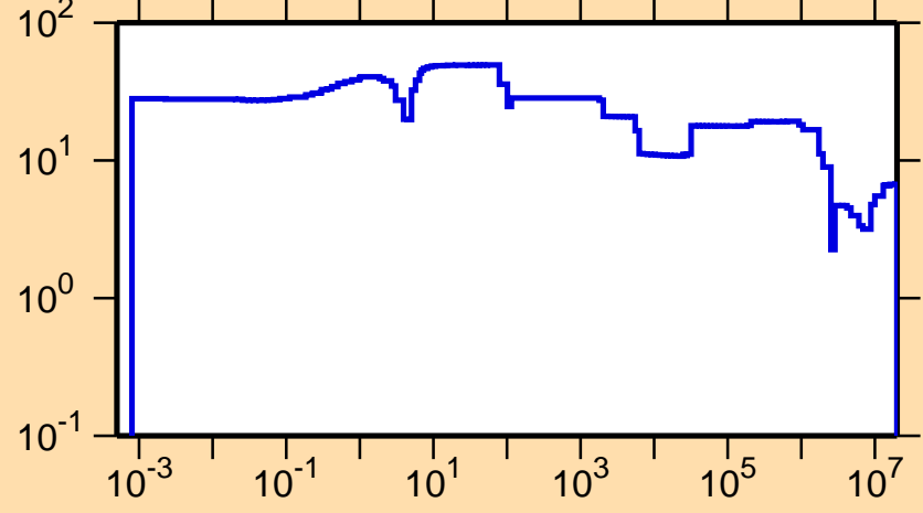
\Delta\sigma/\sigma vs. E for ^{88}\text{Y}(n,\text{tot.})
