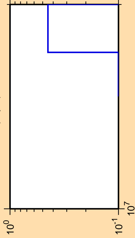
\Delta\sigma/\sigma vs. E for ^{89}\text{Y}(n,\text{pd})
