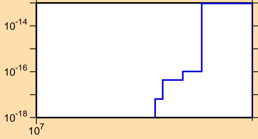
\sigma vs. E for ^{89}\text{Y}(n,\text{pd})
