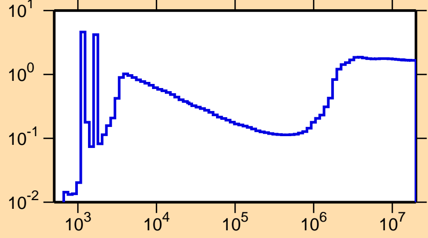
\sigma vs. E for ^{89}\text{Y}(n,\text{nonel.})
