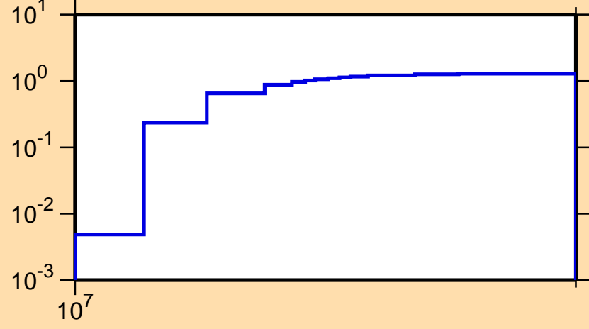
\sigma vs. E for ^{89}\text{Y}(n,2n)
