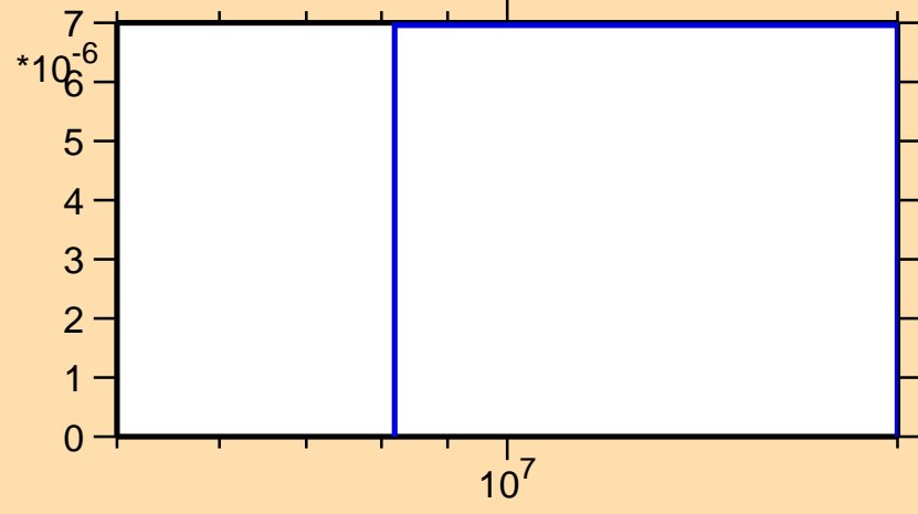
\sigma vs. E for ^{89}\text{Y}(n,t)
