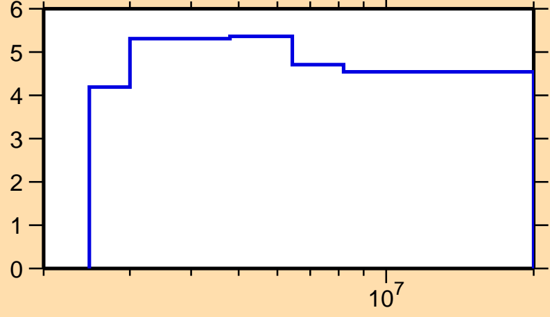
\Delta\sigma/\sigma vs. E for ^{89}\text{Y}(n,\text{nonel.})
