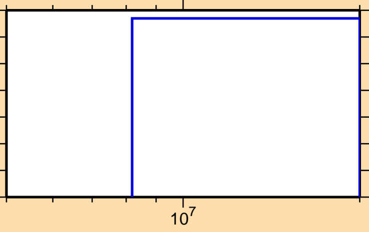
\sigma vs. E for ^{90}\text{Y}(n,\text{He}3)
