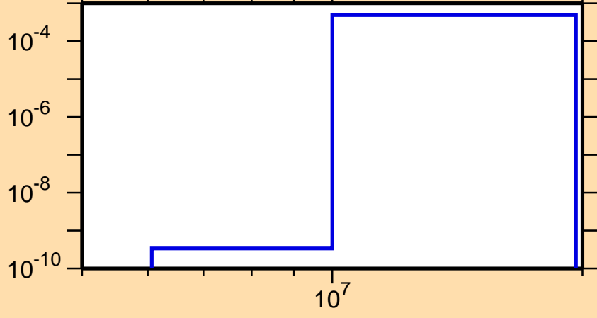
\sigma vs. E for ^{91}\text{Y}(n,n\alpha)
