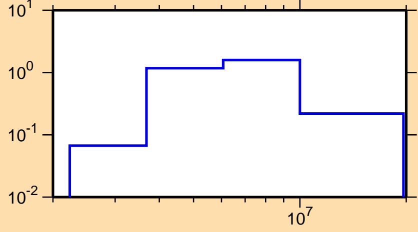
\sigma vs. E for ^{91}\text{Y}(n,n\text{cont.})
