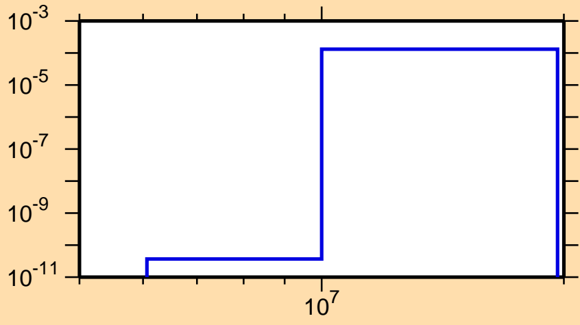
\sigma vs. E for ^{91}\text{Y}(n,t)
