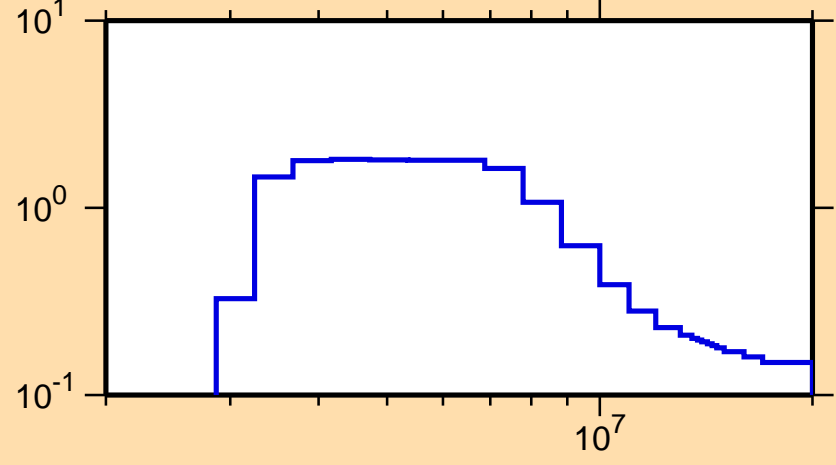
\sigma vs. E for ^{92}\text{Y}(n,n\text{cont.})
