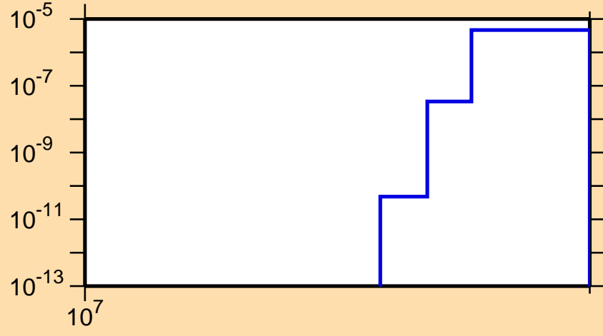
\sigma vs. E for ^{92}\text{Y}(n,2np)
