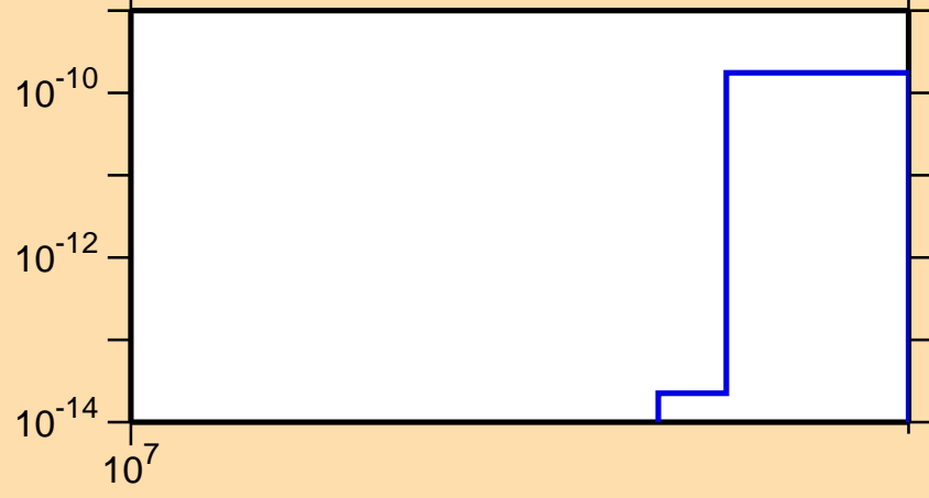
\sigma vs. E for ^{92}\text{Y}(n,\text{He}3)
