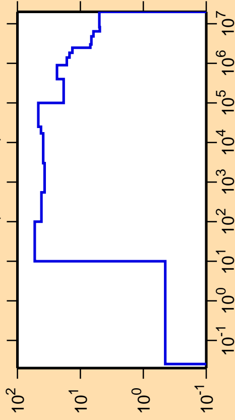
\Delta\sigma/\sigma vs. E for ^{92}\text{Y}(n,\text{nonel.})
