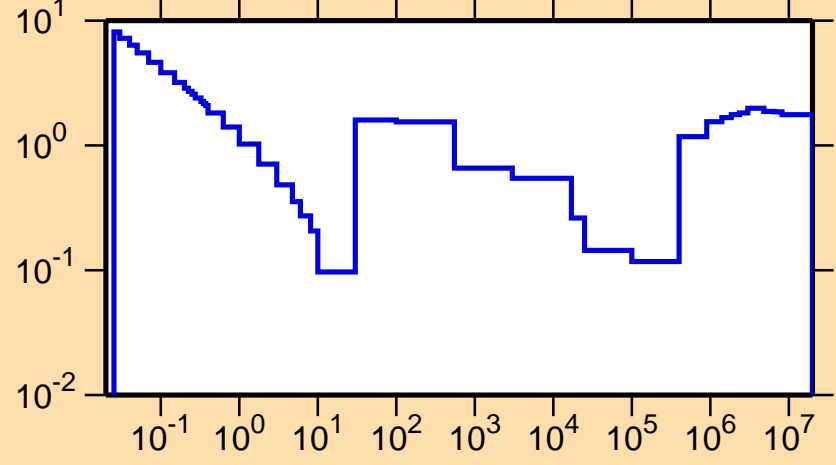
\sigma vs. E for ^{92}\text{Y}(n,\text{nonel.})
