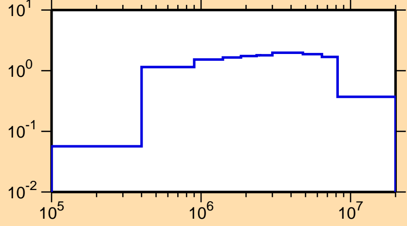
\sigma vs. E for ^{92}\text{Y}(n,\text{inel.})
