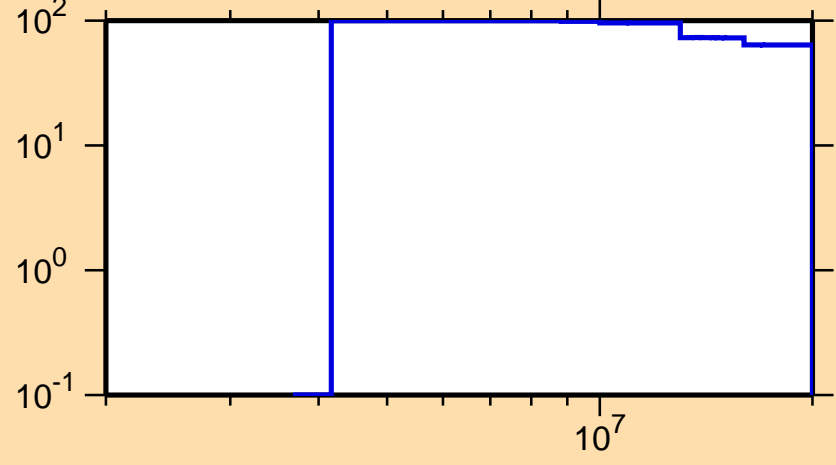
\Delta\sigma/\sigma vs. E for ^{93}\text{Y}(n,p)
