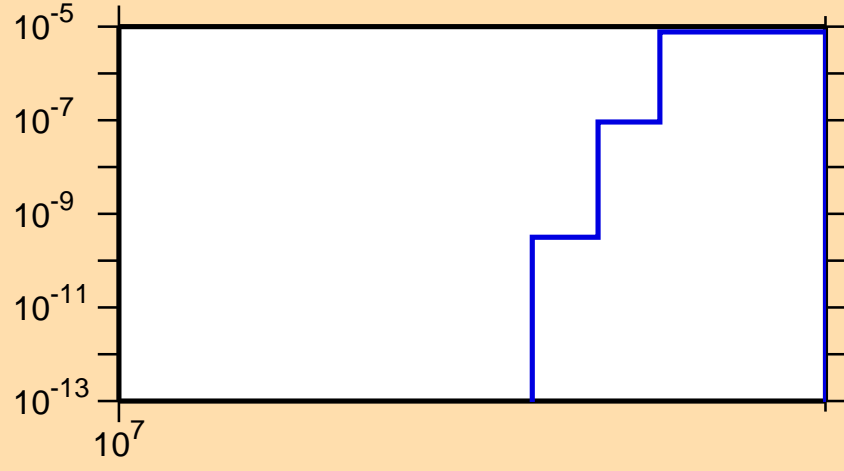
\sigma vs. E for ^{93}\text{Y}(n,nd)
