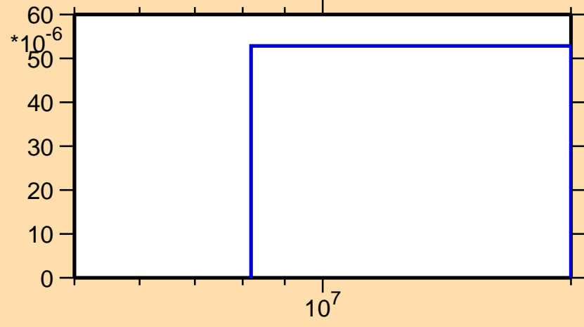
\sigma vs. E for ^{93}\text{Y}(n,t)
