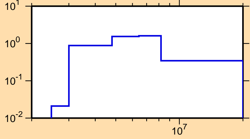
\sigma vs. E for ^{93}\text{Y}(n,n\text{cont.})
