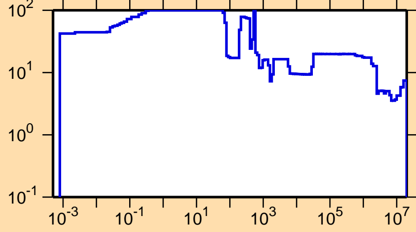
\Delta\sigma/\sigma vs. E for ^{94}\text{Y}(n,\text{tot.})
