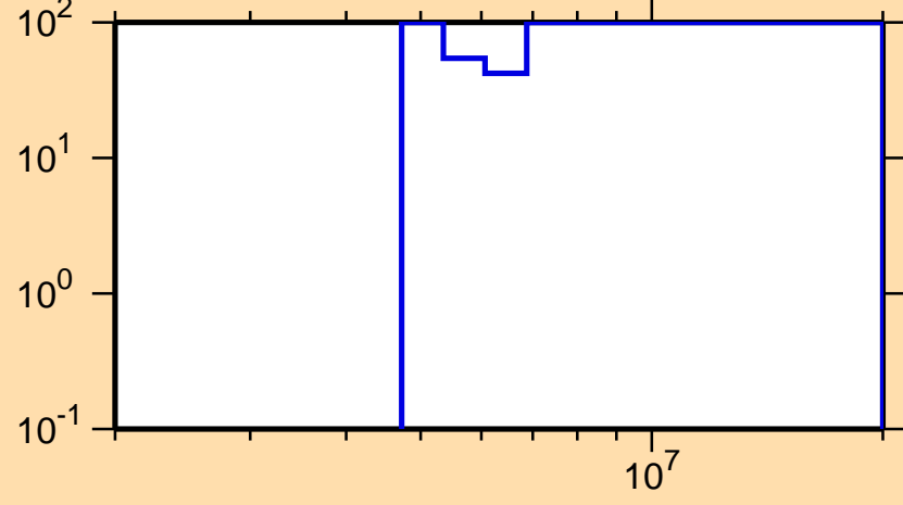
\Delta\sigma/\sigma vs. E for ^{94}\text{Y}(n,ncont.)
