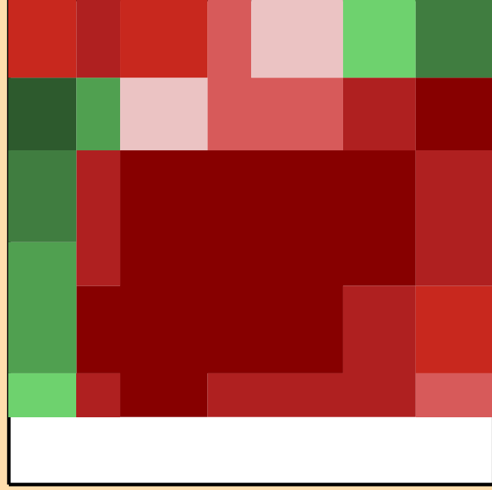
\Delta\sigma/\sigma vs. E for ^{94}\text{Y}(n,\text{inel.})
