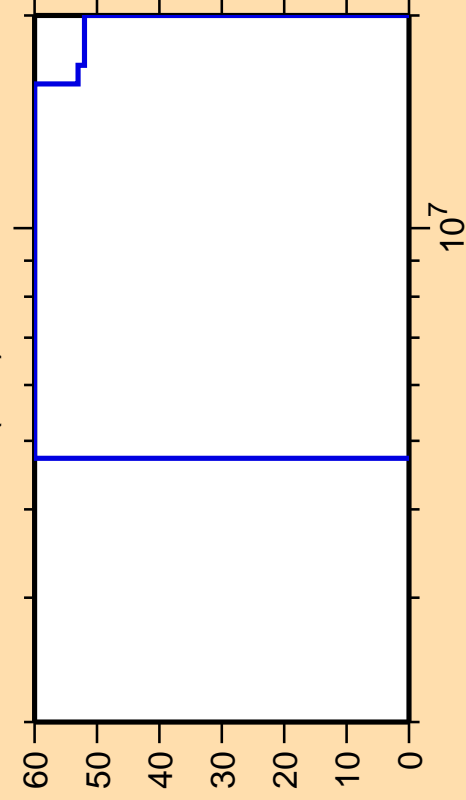
\Delta\sigma/\sigma vs. E for ^{94}\text{Y}(n,\alpha)
