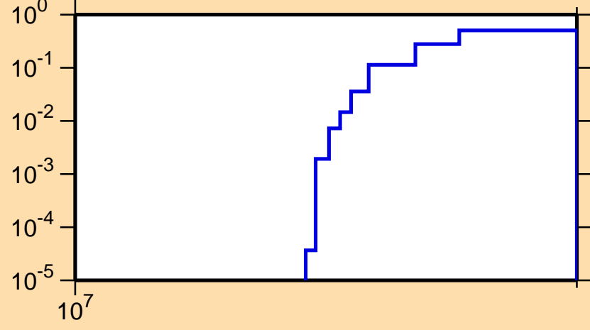
\sigma vs. E for ^{94}\text{Y}(n,3n)
