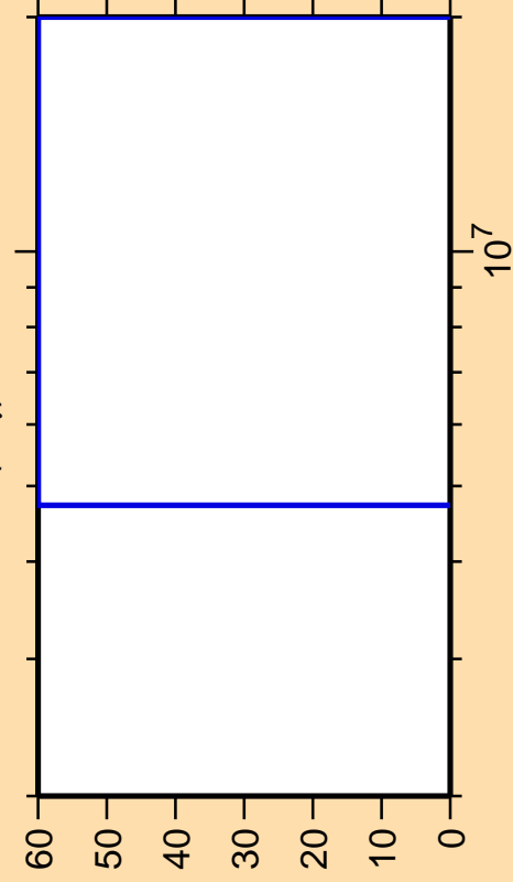
\Delta\sigma/\sigma vs. E for ^{94}\text{Y}(n,\gamma)
