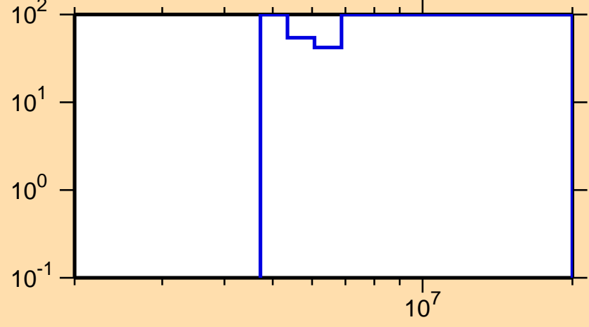
\Delta\sigma/\sigma vs. E for ^{94}\text{Y}(n,n\text{cont.})
