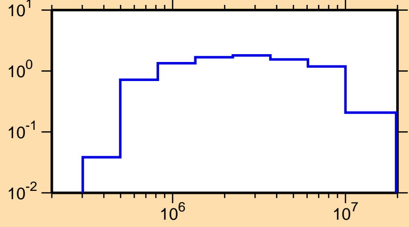
\sigma vs. E for ^{94}\text{Y}(n,\text{inel.})
