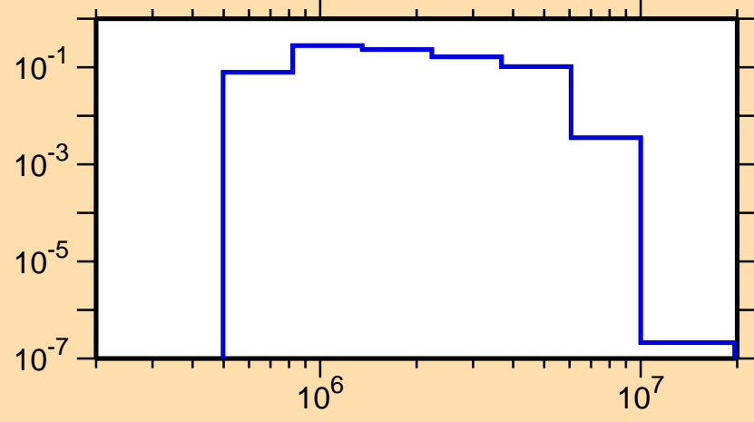
\sigma vs. E for ^{94}\text{Y}(n,n_2)
