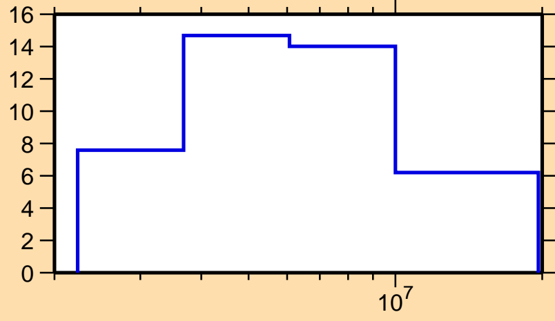
\Delta\sigma/\sigma vs. E for ^{94}\text{Y}(n,el.)
