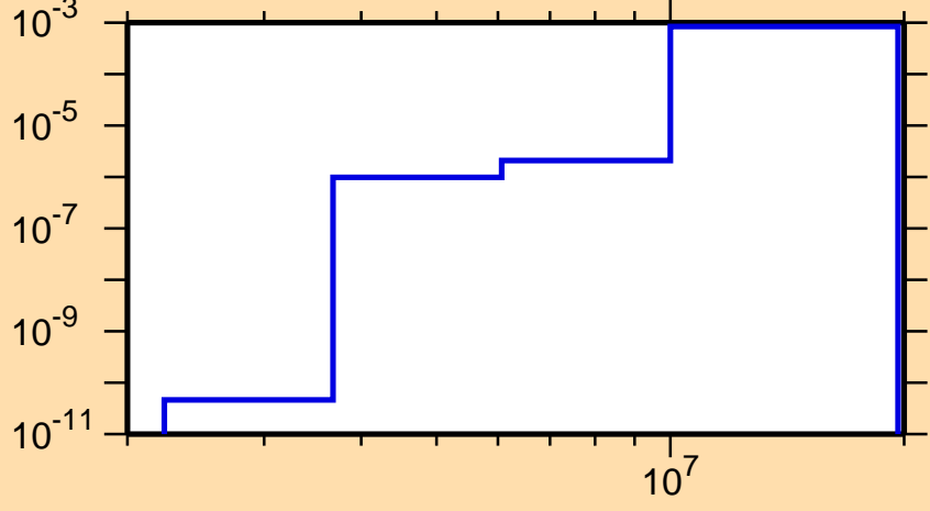
\sigma vs. E for ^{94}\text{Y}(n,\alpha)
