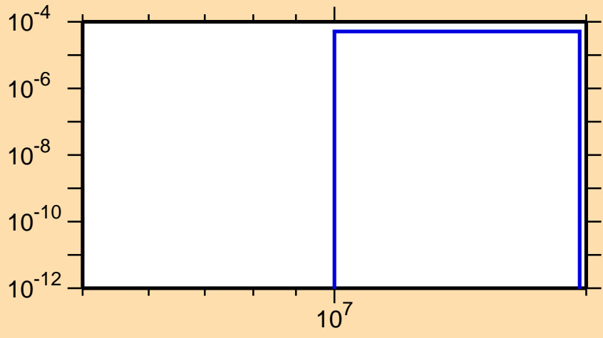
\sigma vs. E for ^{94}\text{Y}(n,n\alpha)
