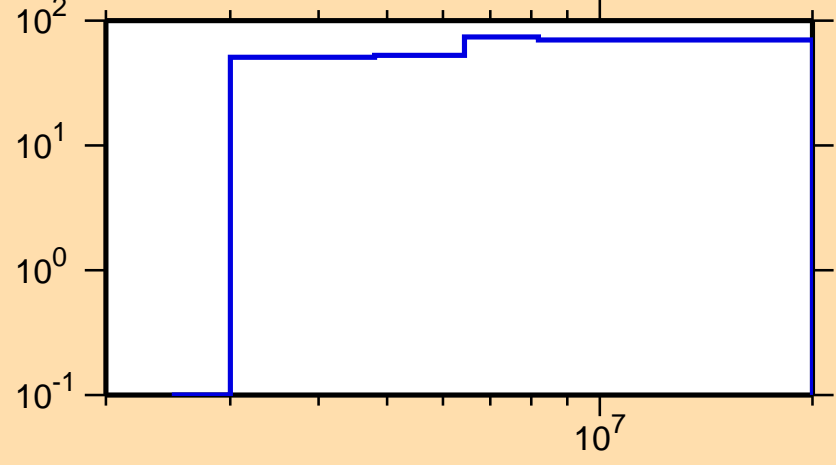
\Delta\sigma/\sigma vs. E for ^{94}\text{Y}(n,p)
