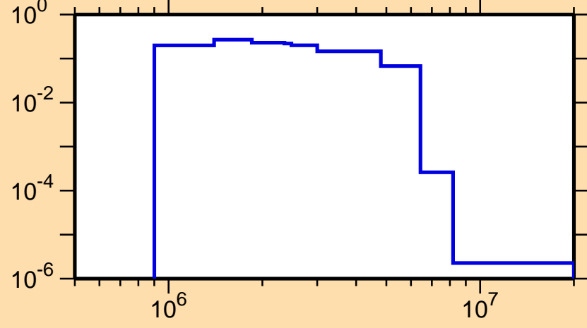
\sigma vs. E for ^{94}\text{Y}(n,n_4)
