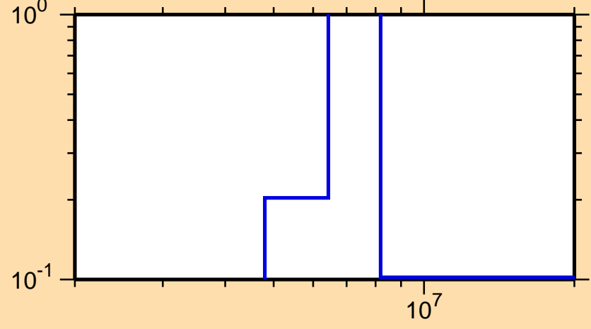
\sigma vs. E for ^{94}\text{Y}(n,n\text{cont.})
