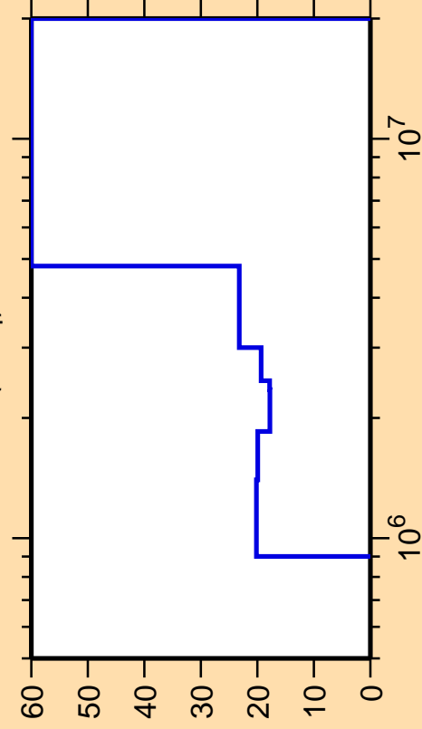
\Delta\sigma/\sigma vs. E for ^{94}\text{Y}(n,n_4)
