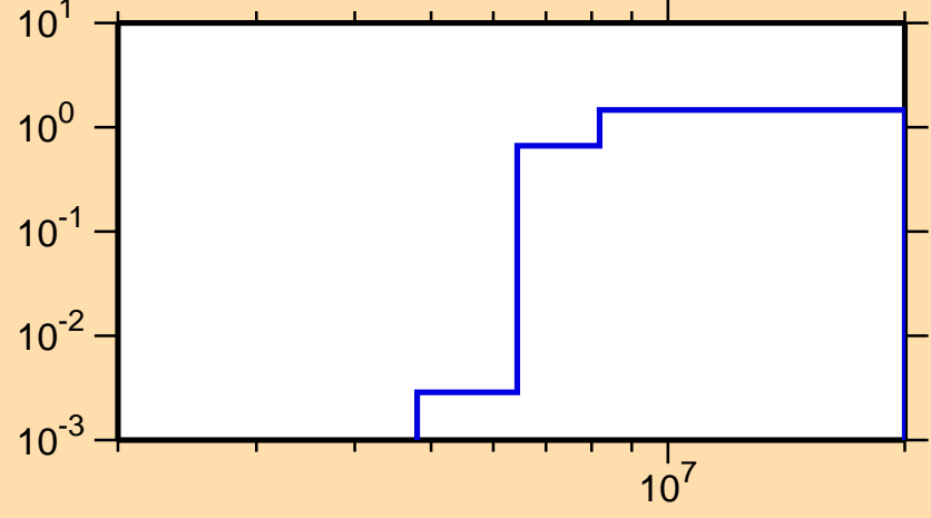
\sigma vs. E for ^{94}\text{Y}(n,2n)
