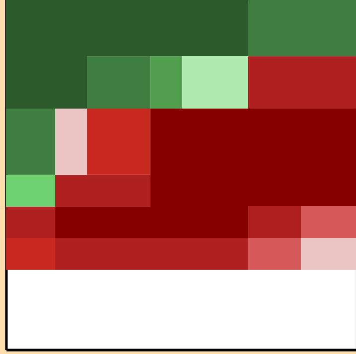
\Delta\sigma/\sigma vs. E for ^{95}\text{Y}(n,\text{inel.})
