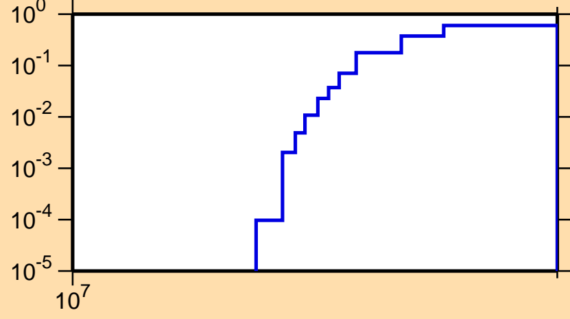
\sigma vs. E for ^{95}\text{Y}(n,3n)
