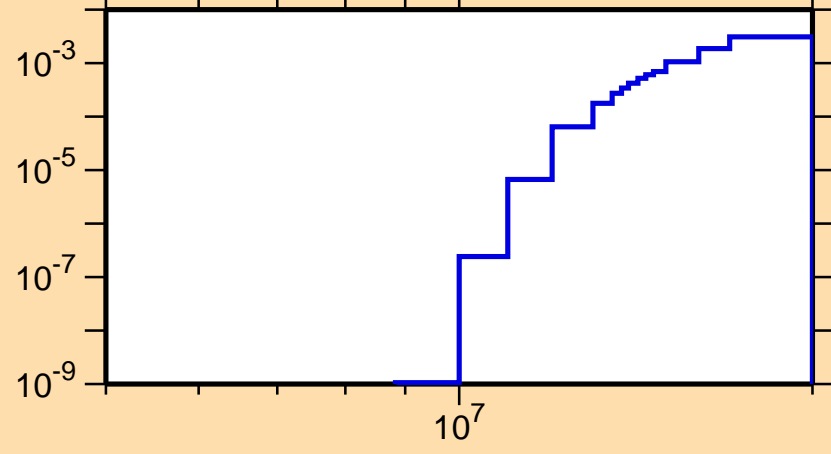
\sigma vs. E for ^{95}\text{Y}(n,d)
