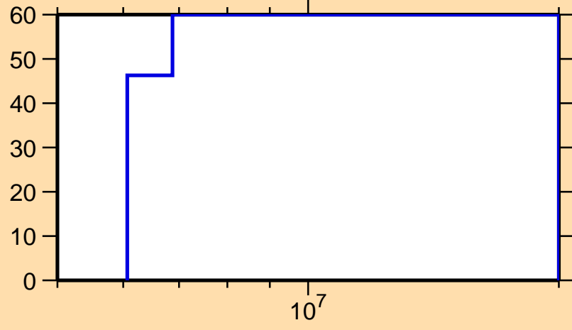
\Delta\sigma/\sigma vs. E for ^{95}\text{Y}(n,n\text{cont.})
