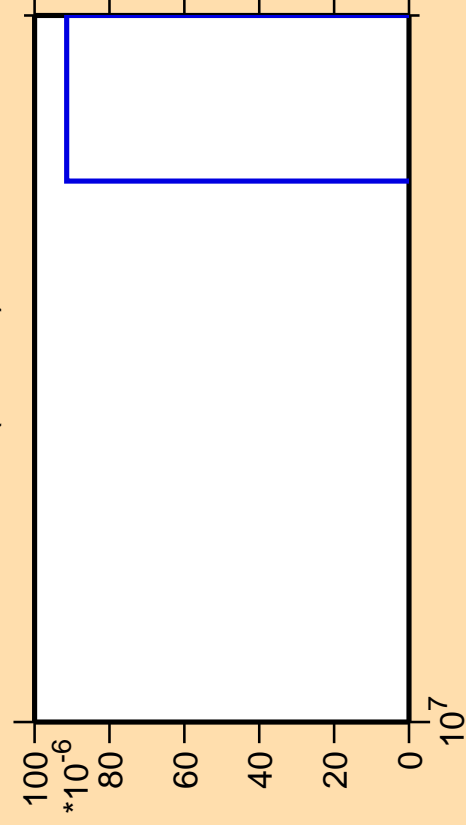
\Delta\sigma/\sigma vs. E for ^{95}\text{Y}(n,3n\alpha)
