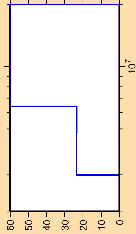
\Delta\sigma/\sigma vs. E for ^{95}\text{Y}(n,ncont.)
