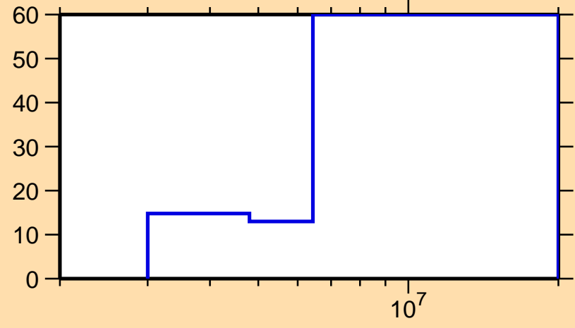
\Delta\sigma/\sigma vs. E for ^{95}\text{Y}(n,incl.)
