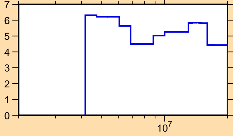
\Delta\sigma/\sigma vs. E for ^{96}\text{Y}(n,\text{nonel.})
