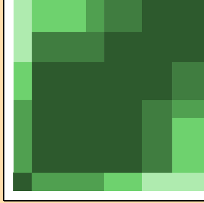
\sigma vs. E for ^{97}\text{Y}(n,2n)
