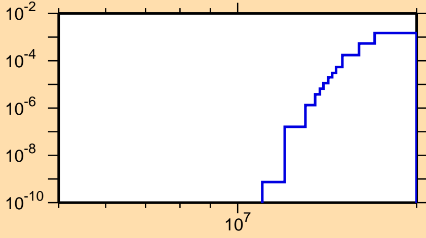
\sigma vs. E for ^{97}\text{Y}(n,np)
