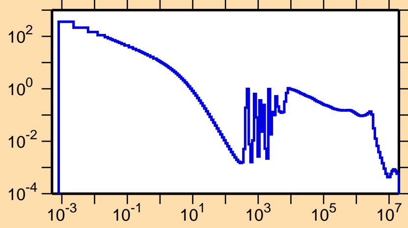
\sigma vs. E for ^{97}\text{Y}(n,\gamma)
