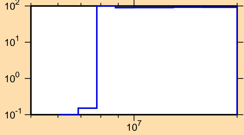
\Delta\sigma/\sigma vs. E for ^{97}\text{Y}(n,p)
