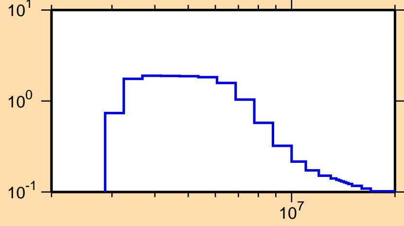
\sigma vs. E for ^{97}\text{Y}(n,n\text{cont.})
