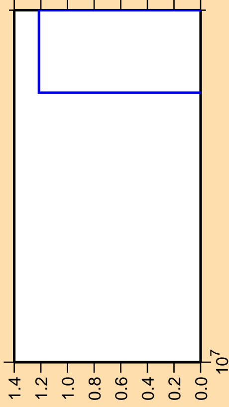
\Delta\sigma/\sigma vs. E for ^{97}\text{Y} (mt 11)
