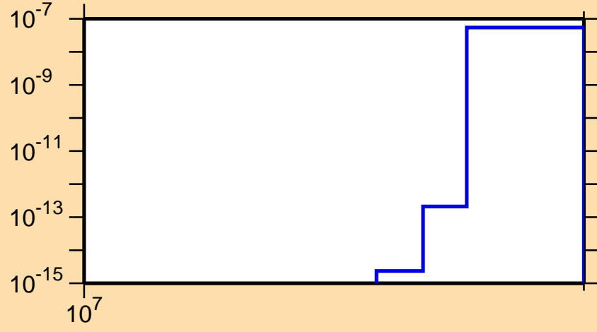
\sigma vs. E for ^{97}\text{Y}(n,2np)
