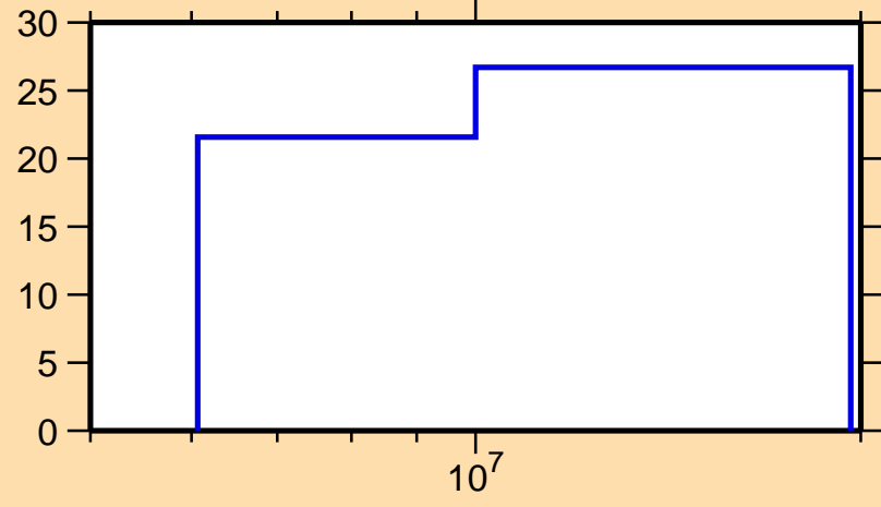
\Delta\sigma/\sigma vs. E for ^{97}\text{Y}(n,el.)
