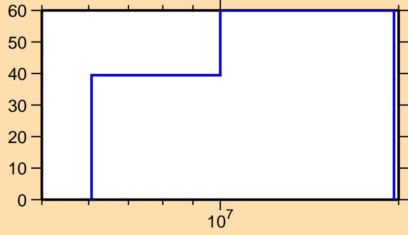
\Delta\sigma/\sigma vs. E for ^{97}\text{Y}(n,ncont.)
