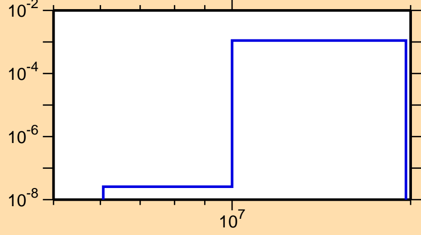
\sigma vs. E for ^{97}\text{Y}(n,p)
