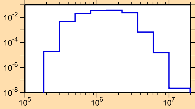
\sigma vs. E for ^{97}\text{Y}(n,n_3)
