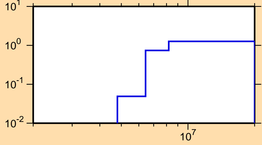
\sigma vs. E for ^{97}\text{Y}(n,2n)
