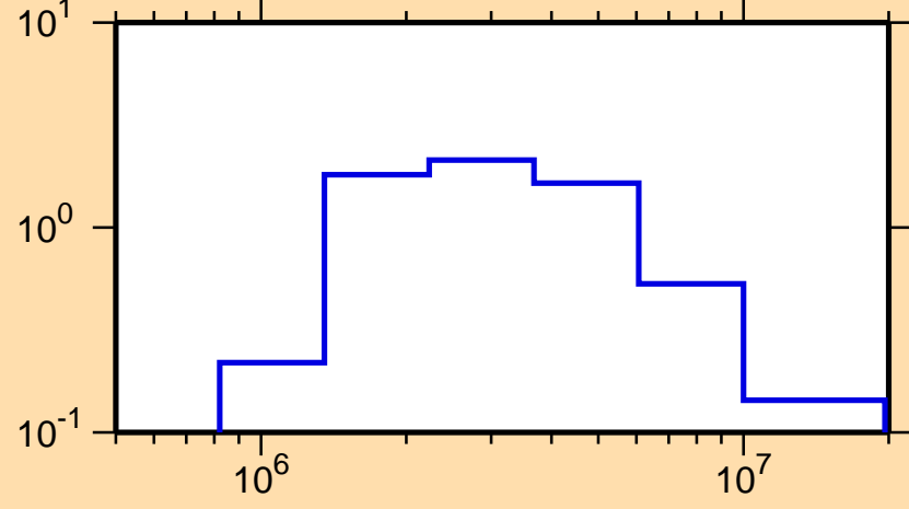
\sigma vs. E for ^{98}\text{Y}(n,n\text{cont.})
