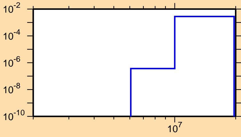
\sigma vs. E for ^{98}\text{Y}(n,p)
