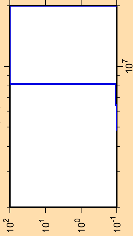
\Delta\sigma/\sigma vs. E for ^{98}\text{Y}(n,t)
