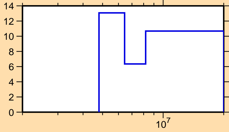
\Delta\sigma/\sigma vs. E for ^{98}\text{Y}(n,el.)
