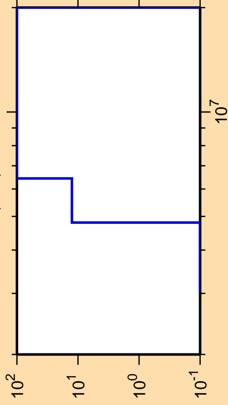
\Delta\sigma/\sigma vs. E for ^{98}\text{Y}(n,\alpha)
