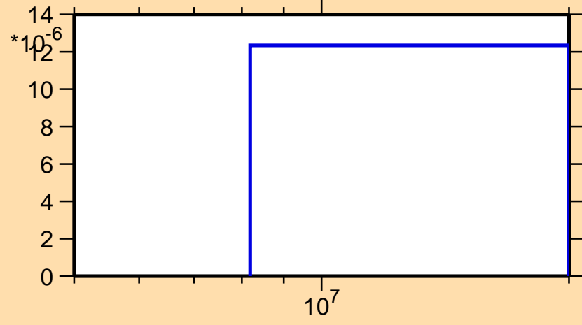
\sigma vs. E for ^{98}\text{Y}(n,n\alpha)
