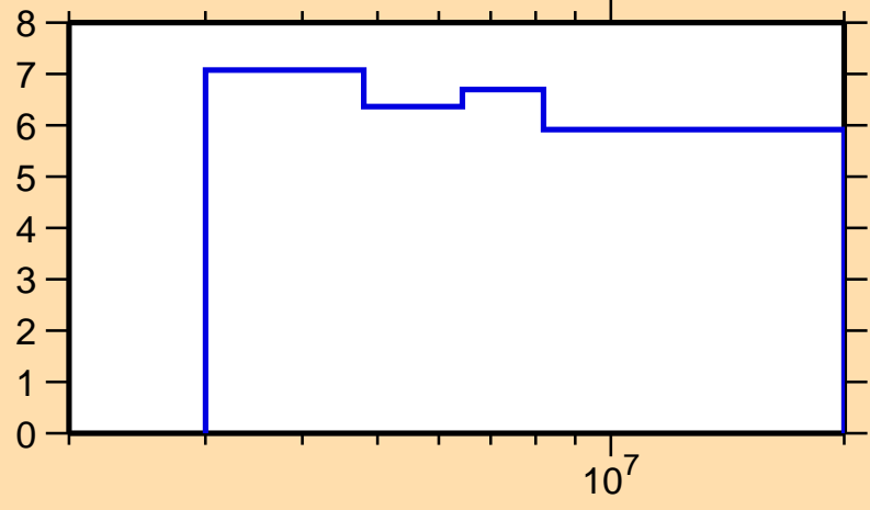
\Delta\sigma/\sigma vs. E for ^{98}\text{Y}(n,\text{nonel.})
