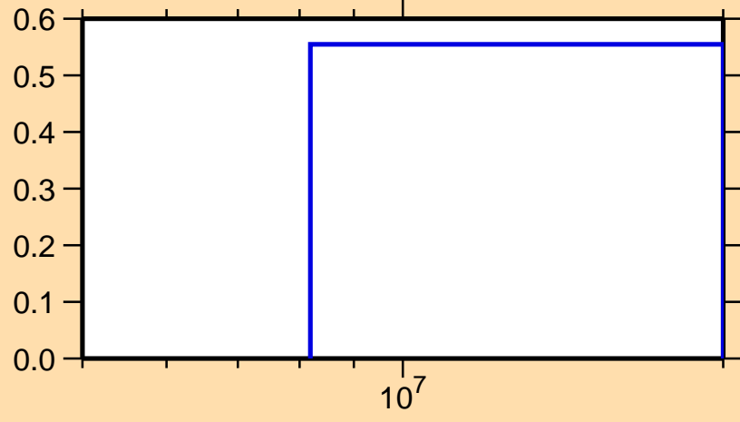
\sigma vs. E for ^{98}\text{Y}(n,3n)
