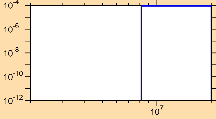
\sigma vs. E for ^{98}\text{Y}(n,t)
