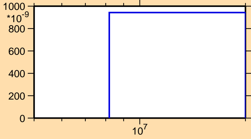
\sigma vs. E for ^{98}\text{Y}(n,nt)
