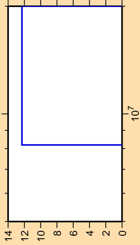
\Delta\sigma/\sigma vs. E for ^{98}\text{Y}(n,3n)
