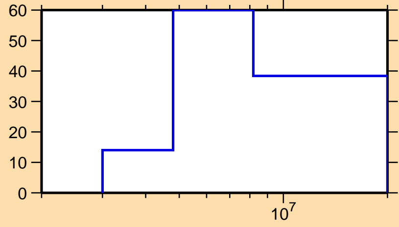
\Delta\sigma/\sigma vs. E for ^{98}\text{Y}(n,n\text{cont.})
