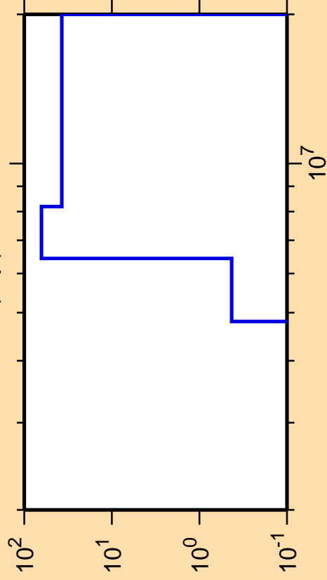
\Delta\sigma/\sigma vs. E for ^{98}\text{Y}(n,p)
