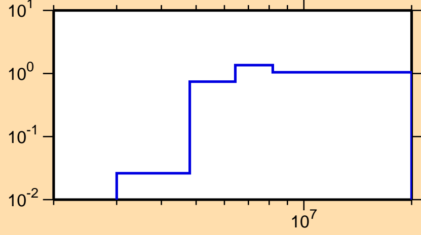
\sigma vs. E for ^{98}\text{Y}(n,2n)
