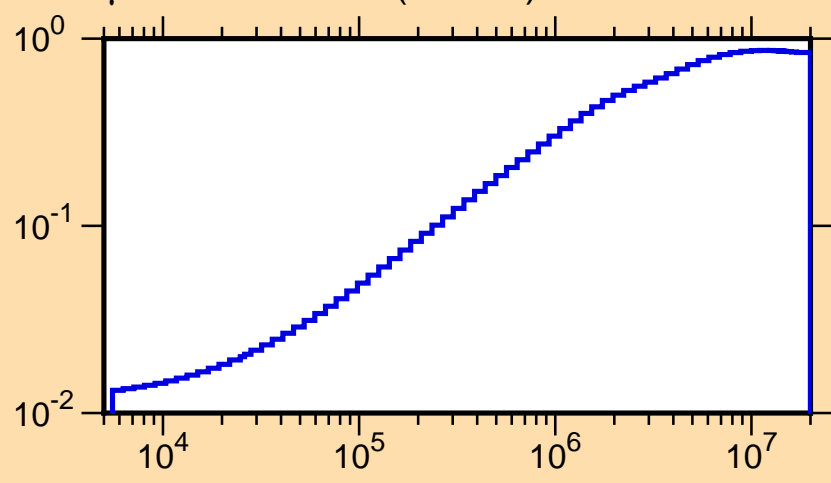
\mu vs. E for ^{60}\text{Zn}(\text{mt251})
