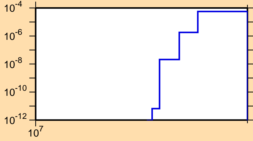
\sigma vs. E for ^{60}\text{Zn}(n,\text{pt})
