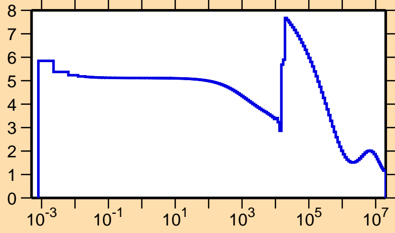
\sigma vs. E for ^{60}\text{Zn}(n,\text{el.})
