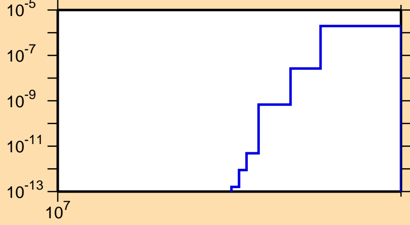
\sigma vs. E for ^{60}\text{Zn} (mt 45)
