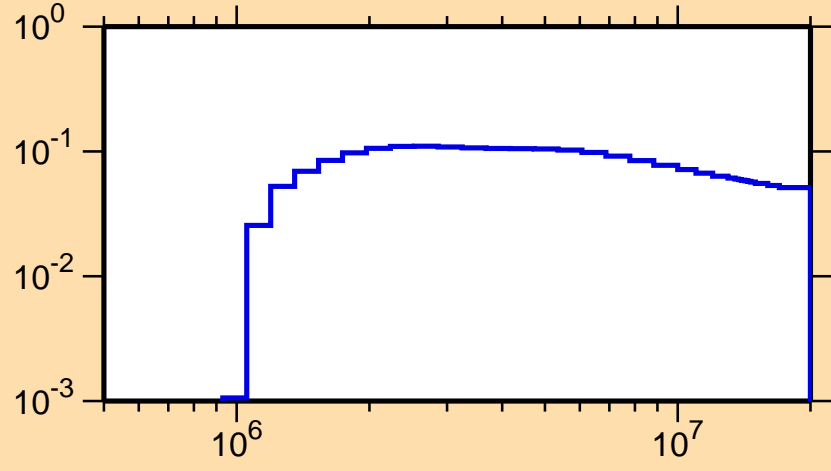
\sigma vs. E for ^{60}\text{Zn}(n,n_1)
