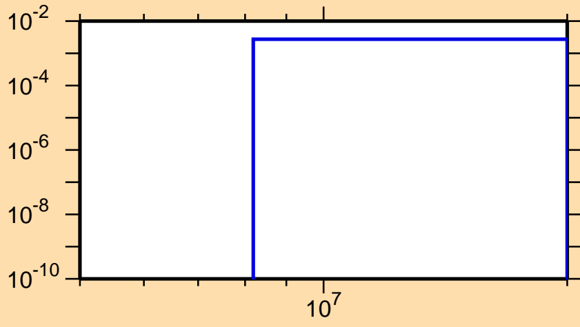
\sigma vs. E for ^{60}\text{Zn}(n,pd)
