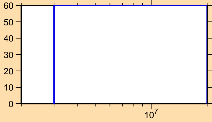
\Delta\sigma/\sigma vs. E for ^{60}\text{Zn}(n,n\text{cont.})
