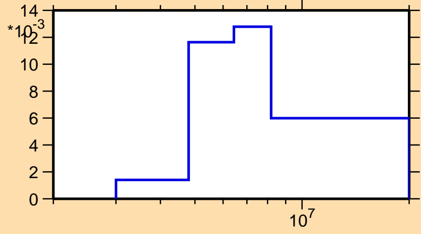
\sigma vs. E for ^{60}\text{Zn}(n,n\text{cont.})
