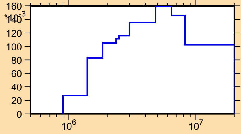
\sigma vs. E for ^{60}\text{Zn}(n,\text{inel.})
