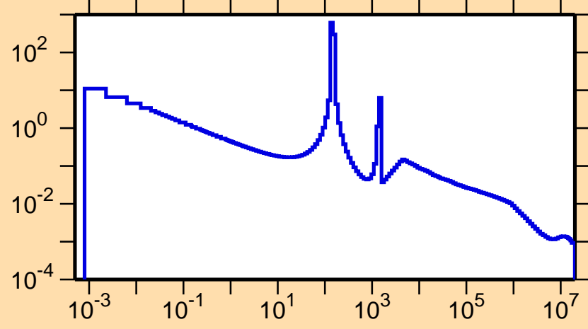
\sigma vs. E for ^{62}\text{Zn}(n,\gamma)
