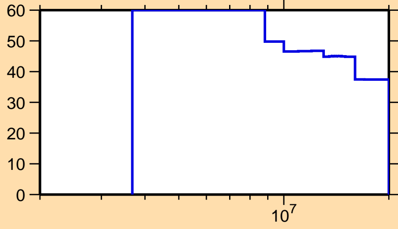
\Delta\sigma/\sigma vs. E for ^{62}\text{Zn}(n,ncont.)
