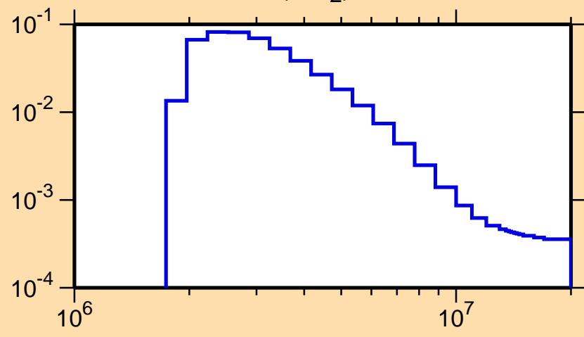
\sigma vs. E for ^{62}\text{Zn}(n,n_2)
