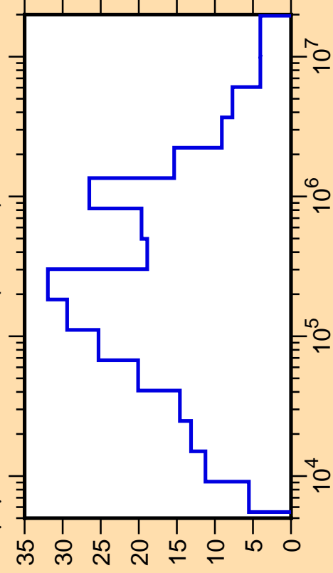
\Delta\mu/\mu vs. E for ^{62}\text{Zn}(\text{mt251})
