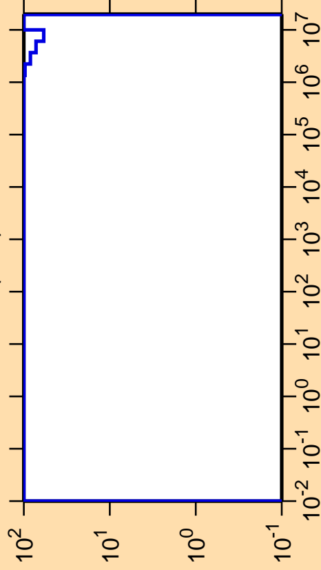
\Delta\sigma/\sigma vs. E for ^{62}\text{Zn}(n,\alpha)
