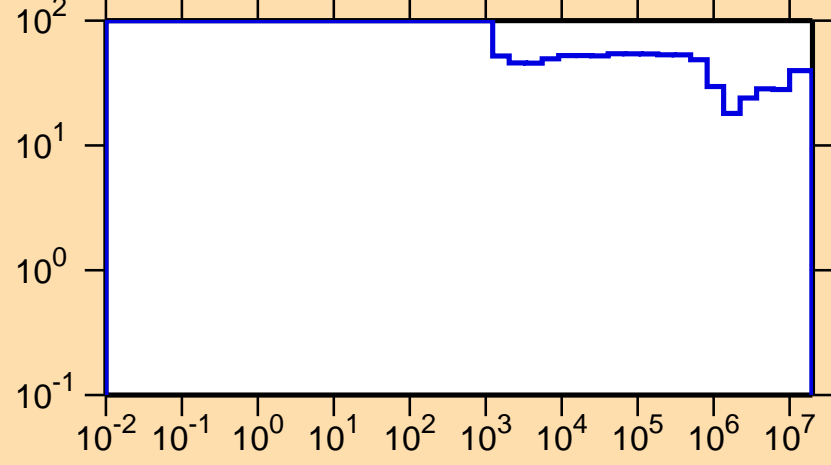
\Delta\sigma/\sigma vs. E for ^{62}\text{Zn}(n,p)
