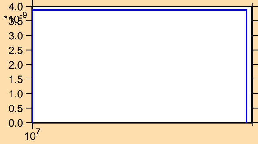
\sigma vs. E for ^{62}\text{Zn}(\text{mt117})
