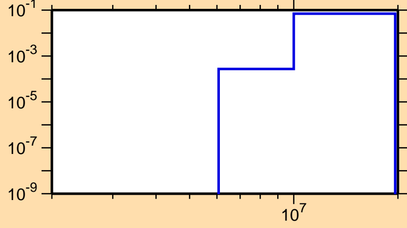
\sigma vs. E for ^{62}\text{Zn}(n,n\alpha)
