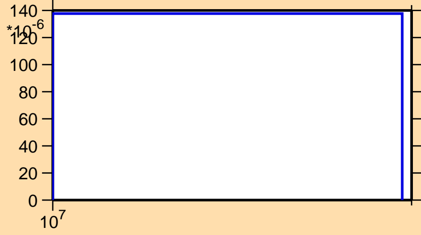
\sigma vs. E for ^{62}\text{Zn}(n,pd)
