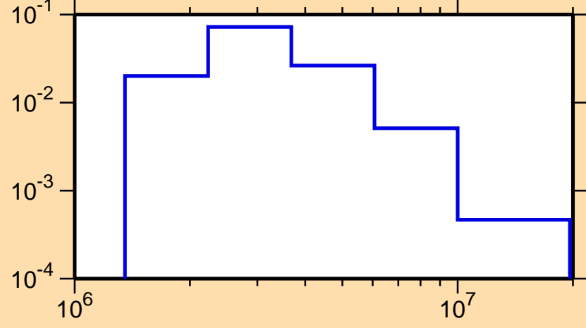
\sigma vs. E for ^{62}\text{Zn}(n,n_2)
