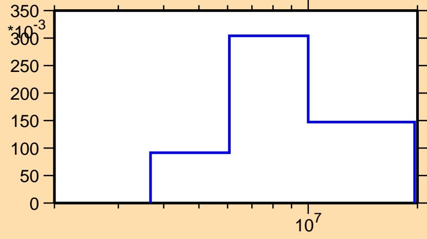
\sigma vs. E for ^{62}\text{Zn}(n,n\text{cont.})
