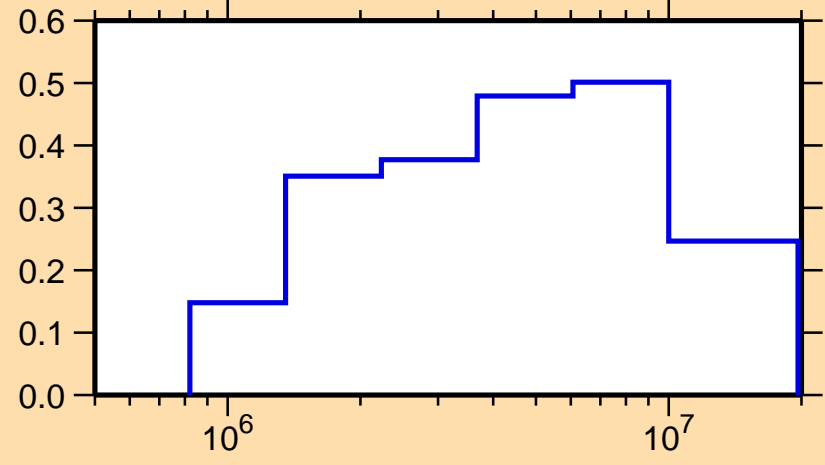
\sigma vs. E for ^{62}\text{Zn}(n,\text{inel.})
