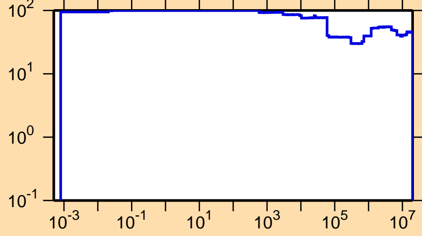
\Delta\sigma/\sigma vs. E for ^{63}\text{Zn}(n,p)
