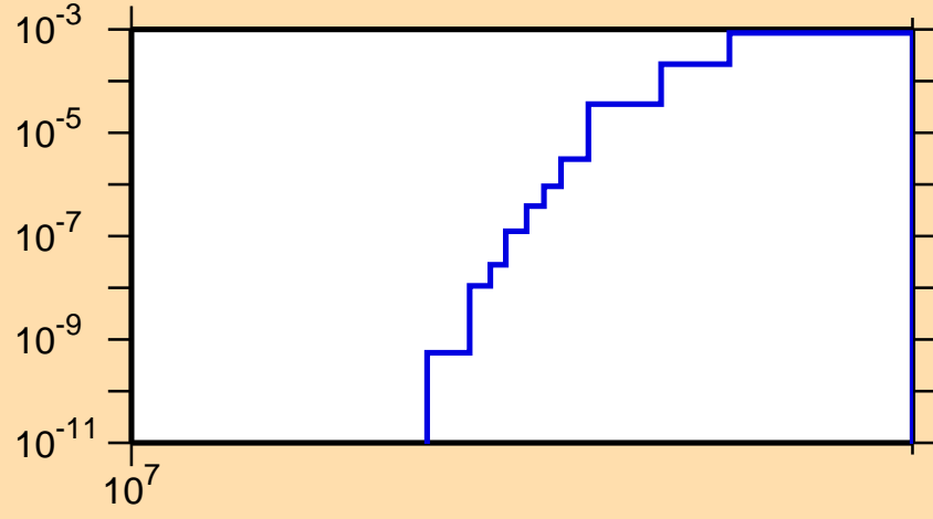
\sigma vs. E for ^{63}\text{Zn}(n,pd)
