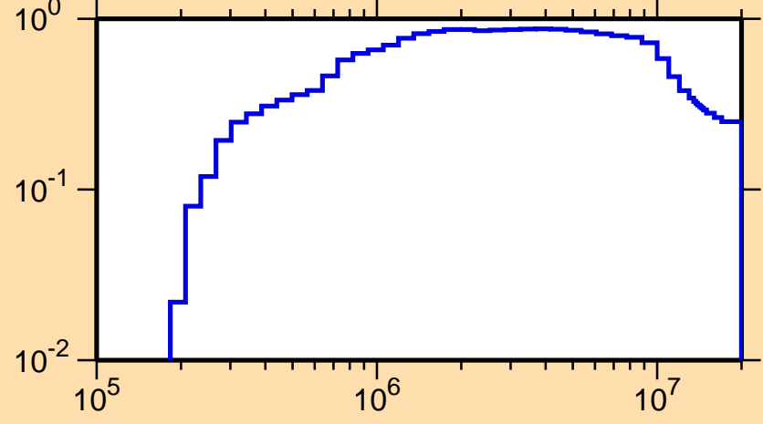
\sigma vs. E for ^{63}\text{Zn}(n,\text{inel.})
