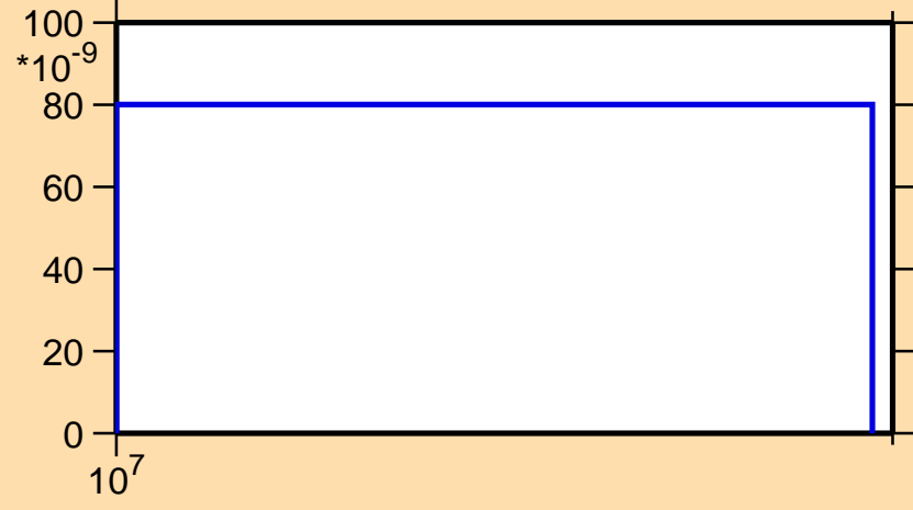
\sigma vs. E for ^{63}\text{Zn}(n,2n\alpha)
