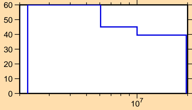
\Delta\sigma/\sigma vs. E for ^{63}\text{Zn}(n,n\text{cont.})
