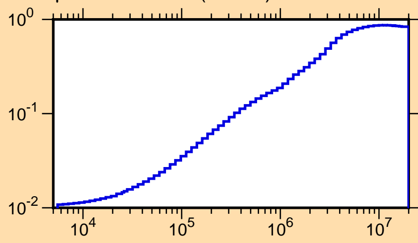
\mu vs. E for ^{66}\text{Zn}(\text{mt251})
