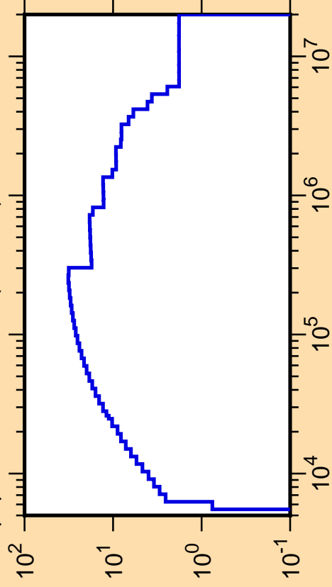
\Delta\mu/\mu vs. E for ^{66}\text{Zn}(\text{mt251})
