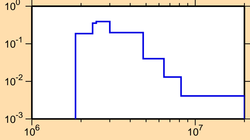
\sigma vs. E for ^{66}\text{Zn}(n,n_2)
