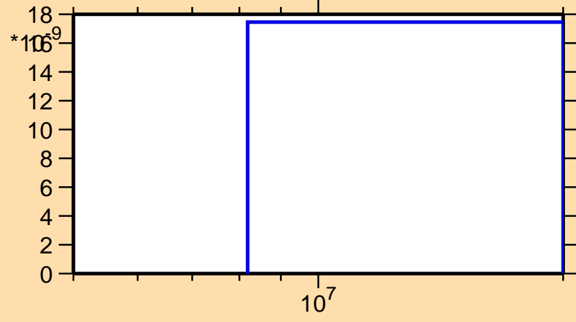
\sigma vs. E for ^{66}\text{Zn}(n,3n)
