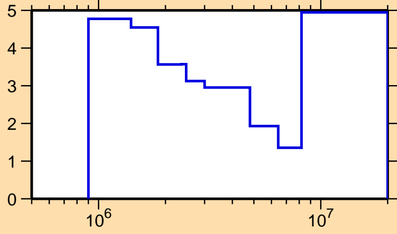
\Delta\sigma/\sigma vs. E for ^{66}\text{Zn}(n,\text{inel.})
