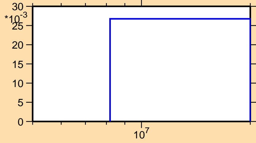
\sigma vs. E for ^{66}\text{Zn}(n,np)
