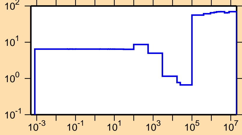
\Delta\sigma/\sigma vs. E for ^{66}\text{Zn}(n,\gamma)
