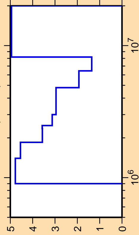
\Delta\sigma/\sigma vs. E for ^{66}\text{Zn}(n,\text{inel.})
