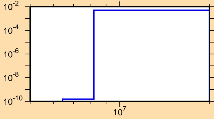
\sigma vs. E for ^{66}\text{Zn}(n,d)
