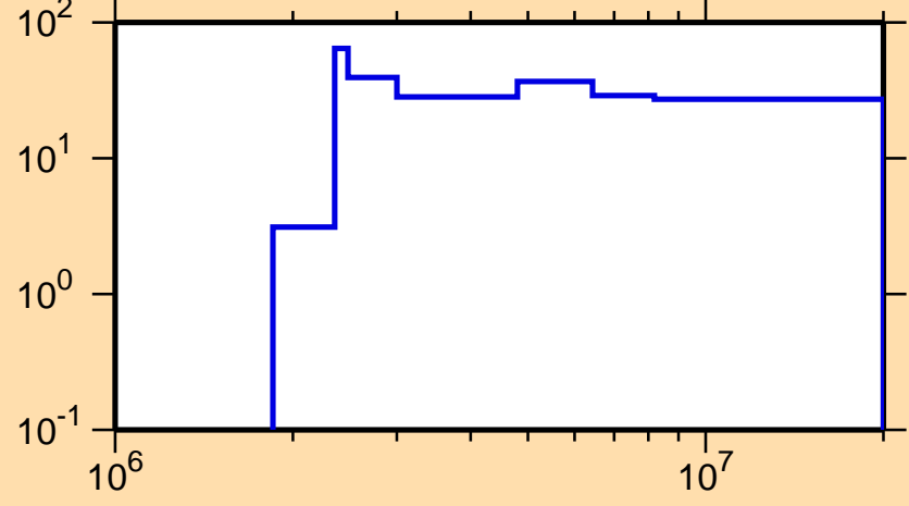
\Delta\sigma/\sigma vs. E for ^{66}\text{Zn}(n,p)
