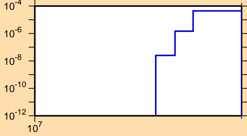
\sigma vs. E for ^{67}\text{Zn}(n,\text{nd})
