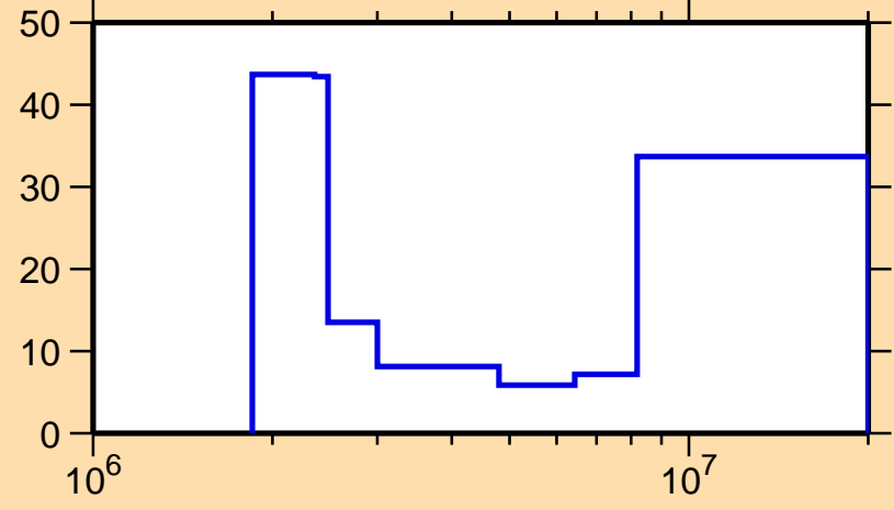
\Delta\sigma/\sigma vs. E for ^{67}\text{Zn}(n,ncont.)
