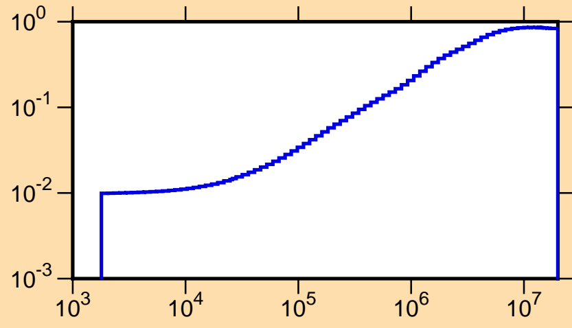
\mu vs. E for ^{69}\text{Zn}(\text{mt251})
