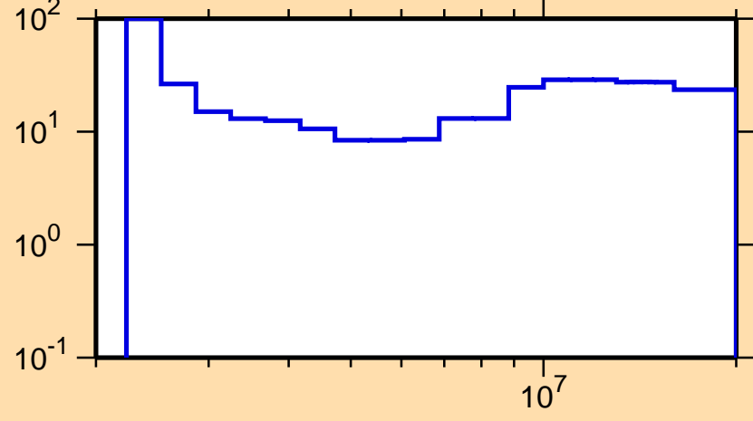
\Delta\sigma/\sigma vs. E for ^{69}\text{Zn}(n,n\text{cont.})
