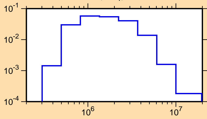
\sigma vs. E for ^{69}\text{Zn}(n,n_1)
