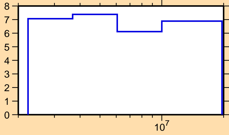
\Delta\sigma/\sigma vs. E for ^{69}\text{Zn}(n,n\text{onel.})
