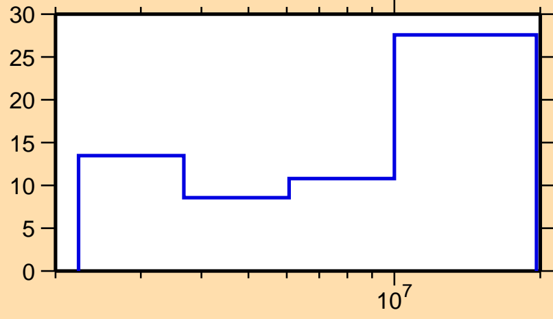
\Delta\sigma/\sigma vs. E for ^{69}\text{Zn}(n,n\text{cont.})
