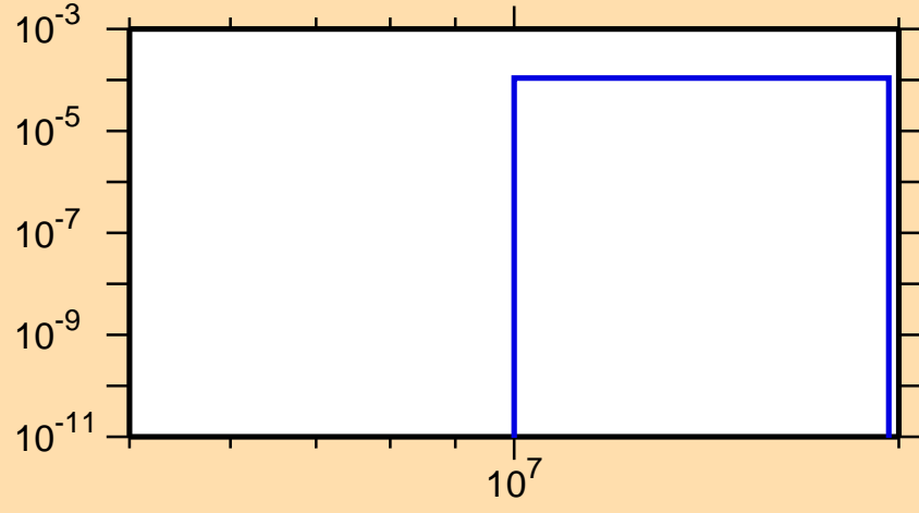
\sigma vs. E for ^{69}\text{Zn}(n,t)
