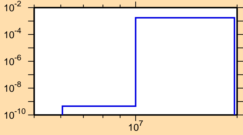
\sigma vs. E for ^{69}\text{Zn}(n,\alpha)
