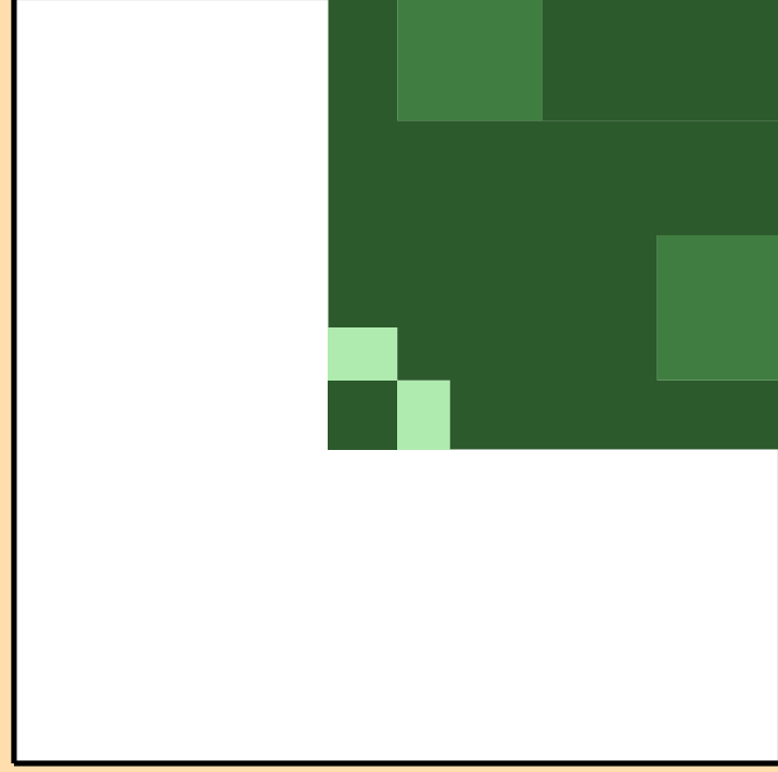
\sigma vs. E for ^{69}\text{Zn}(n,np)
