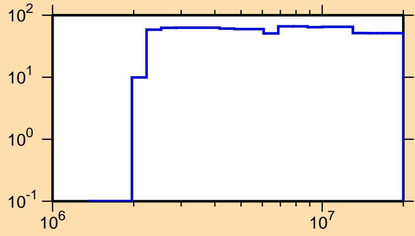
\Delta\sigma/\sigma vs. E for ^{69}\text{Zn}(n,p)
