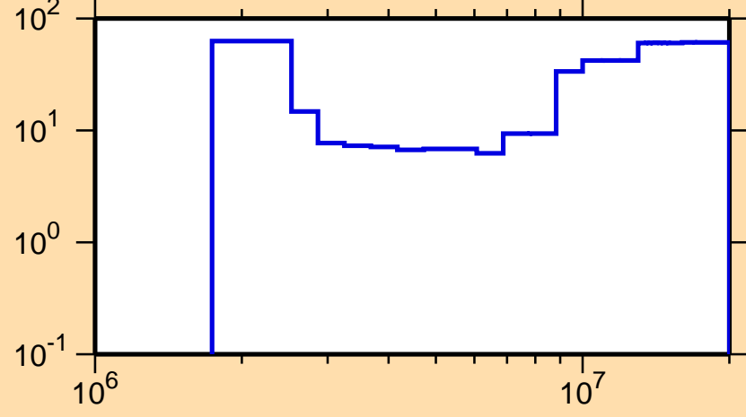
\Delta\sigma/\sigma vs. E for ^{69}\text{Zn}(n,ncont.)
