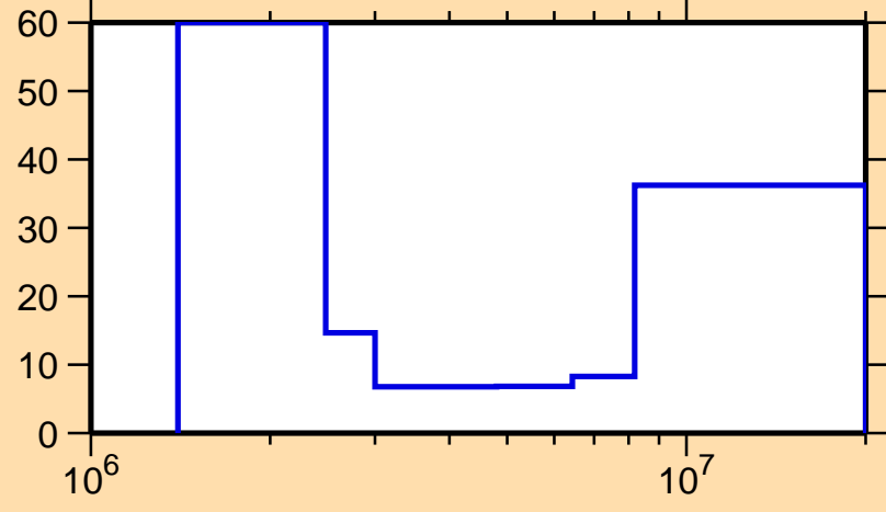
\Delta\sigma/\sigma vs. E for ^{69}\text{Zn}(n,ncont.)
