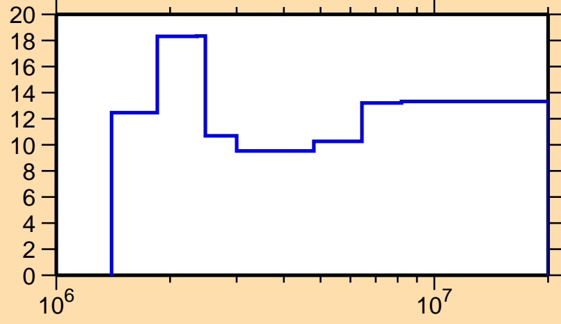
\Delta\sigma/\sigma vs. E for ^{69}\text{Zn}(n,el.)
