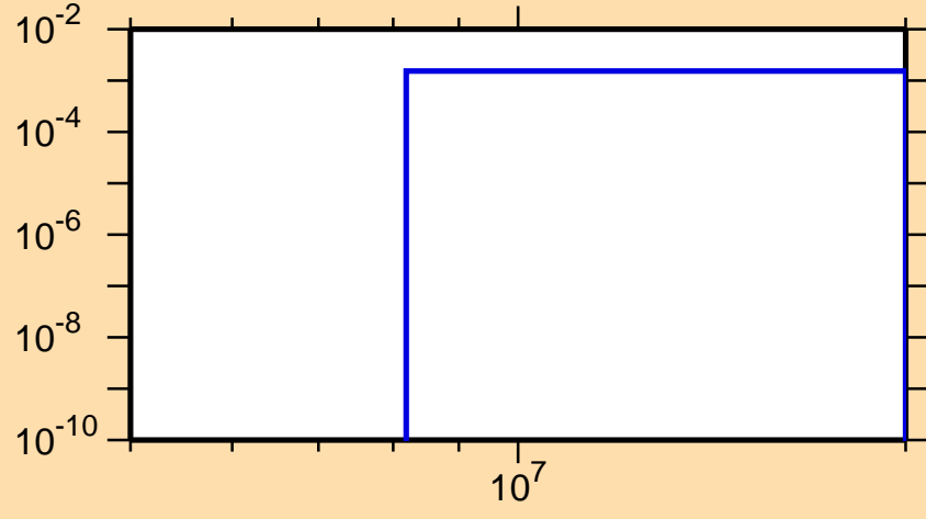
\sigma vs. E for ^{69}\text{Zn}(n,d)
