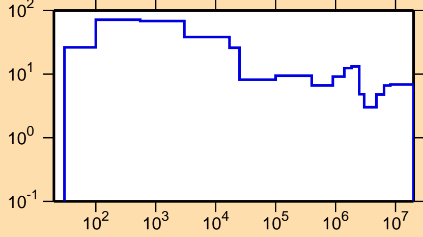
\Delta\sigma/\sigma vs. E for ^{69}\text{Zn}(n,\text{tot.})
