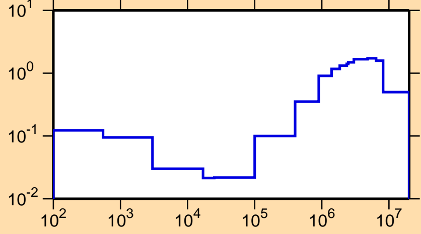
\sigma vs. E for ^{69}\text{Zn}(n,\text{inel.})
