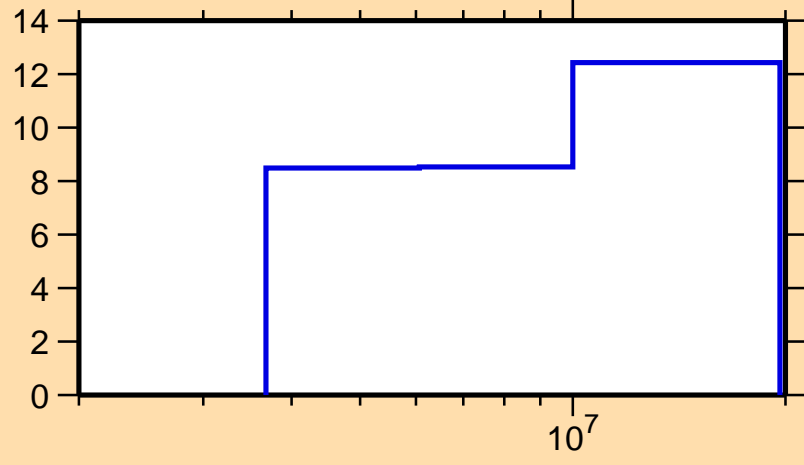
\Delta\sigma/\sigma vs. E for ^{70}\text{Zn}(n,el.)
