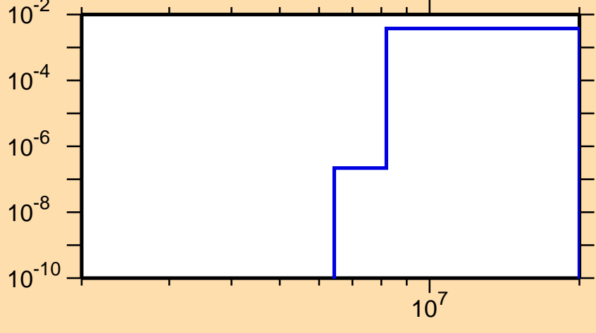
\sigma vs. E for ^{70}\text{Zn}(n,p)
