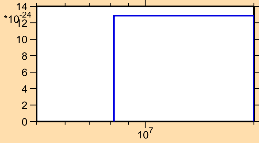
\sigma vs. E for ^{70}\text{Zn}(n,pd)
